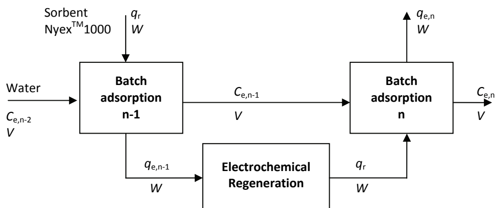
Figure 5. Schematic diagram of two stages in a multi-stage batch adsorption and regeneration system, considered as a multi-stage equilibrium process.
