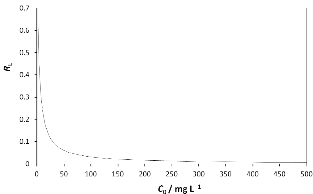
Figure 2. Separation factor for Acid Violet 17 onto the GIC adsorbent Nyex™ 1000 at 20°C.
