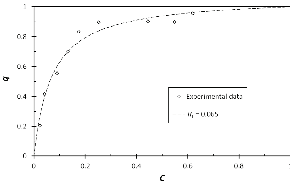
Figure 3. Isotherm shape for adsorption of AV17 onto the GIC adsorbent Nyex™ 1000 at room temperature (23°C) and the curve obtained using Equation (7) with R_L = 0.065 .
