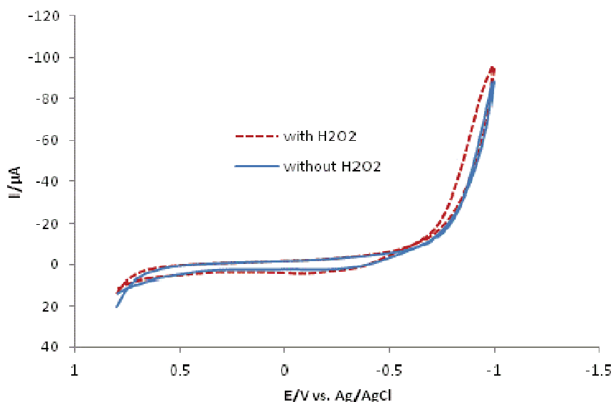
Figure 1. Cyclic voltammograms of \text{H}_2\text{O}_2 at an unmodified CPE; phosphate buffer solution 0.1 M, pH 7.5; Fill curve blank, broken curve with 200 \text{ mg L}^{-1} \text{H}_2\text{O}_2 ; conditions: E_{\text{initial}} = 0.80 \text{ V} , E_{\text{final}} = -1.00 \text{ V} , scan rate 20 \text{ mV s}^{-1} .
