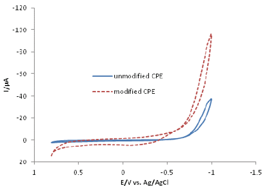
Figure 2. Cyclic voltammogram of a \text{ReO}_2 -modified CPE; E_{\text{initial}} = 0.80 \text{ V} , E_{\text{final}} = -1.0 \text{ V} ; scan rate 20 \text{ mV s}^{-1} ; support electrolyte 0.1 M phosphate buffer, pH 7.5.
