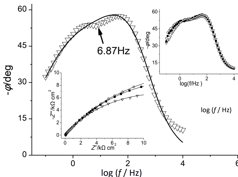
Figure 4. Bode phase diagram of Bi in methanol solution of 0.1 M LiClO 4 at E = 0.15 V vs. Ag|AgCl. Insets: Nyquist and Bode plots at potentials ○ - 0.05, ■ - 0.10 and ▽ - 0.15 V. Lines are fitting results of R(Q[R(RQ)]) equivalent circuit to experimental points.
