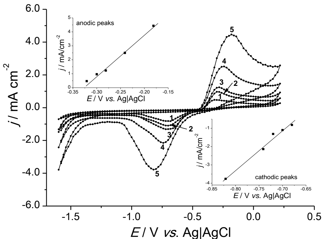
Figure 1. Cyclic voltammograms of Bi in methanol solution of 0.1 M LiClO 4 at various scan rates: (1) 0.025, (2) 0.05, (3) 0.10, (4) 0.20, (5) 0.40 V/s. Insets: Anodic and cathodic peak currents vs. corresponding peak current potentials.
