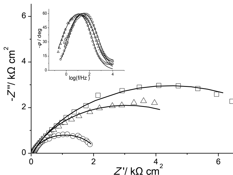
Figure 3. Nyquist plots of Bi in methanol solution of 0.1 M LiClO 4 , at various electrode potentials in V vs. Ag|AgCl: △ -0.4, □ -0.68, ○ -1.4. Inset: Bode phase diagrams at the same potentials. Lines represent simulated responses fitted to experimental points.
