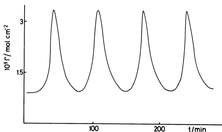
Figure 21. The change in the amount of Cl^- ions in a polypyrrole electrode during four consecutive oxidation-reduction cycles. Solution: 2 \times 10^{-4} \text{ mol dm}^{-3} ^{36}Cl -labeled HCl. Scan rate: 0.4 \text{ mV s}^{-1} . [33]
