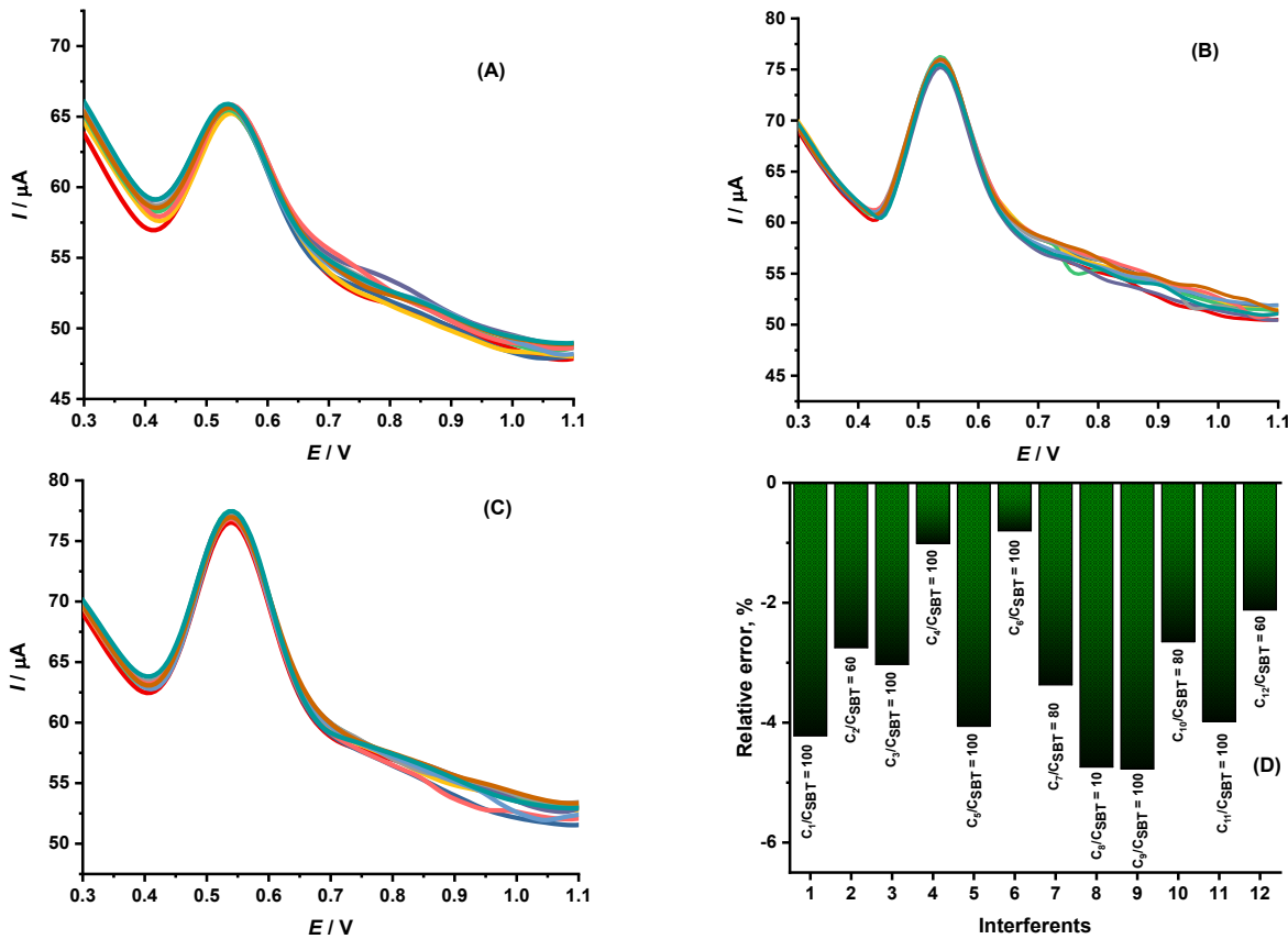
Figure 11. DPVs at (1.0/1)NiF/GrO(S,N)/GCE in BRS 0.1 M (pH 3) with C_{\text{SBT}} , A - 5.0, B - 8.9 and C - 19.6 \mu\text{M} (differently coloured curves represent individual replicate scans recorded under identical experimental conditions) and D - interfering study for 12 substances
