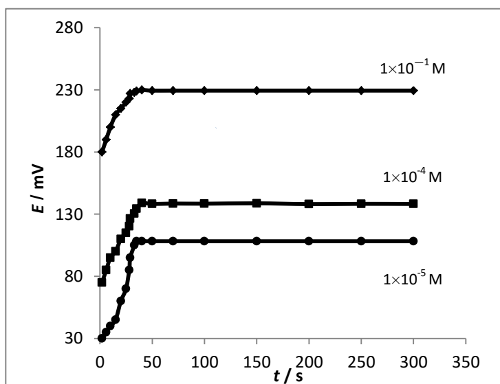
Figure 5. Response time of electrode
