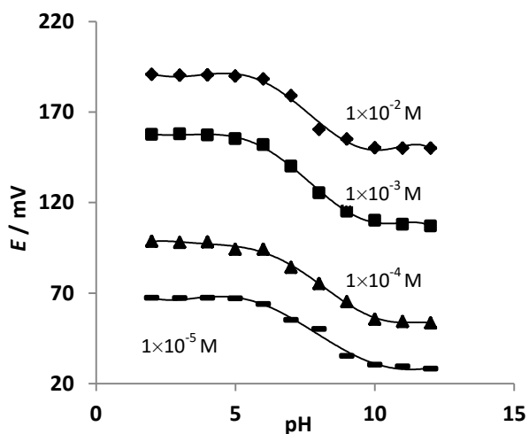
Figure 3. Effect of the pH on the response of the electrode
