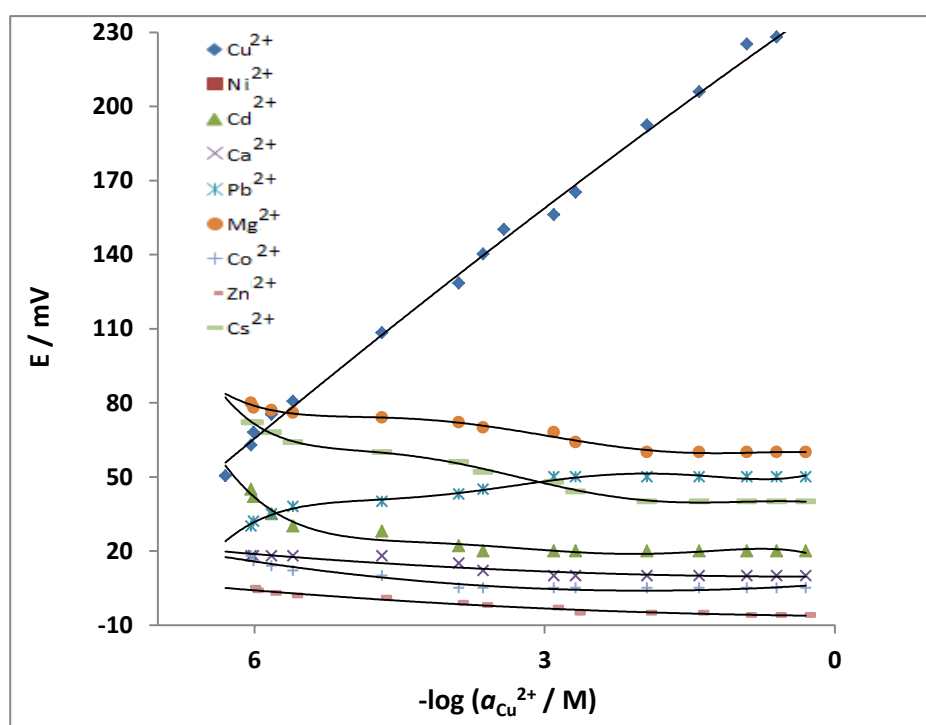
Figure 2. Schematic diagram of electrode response to various cations
