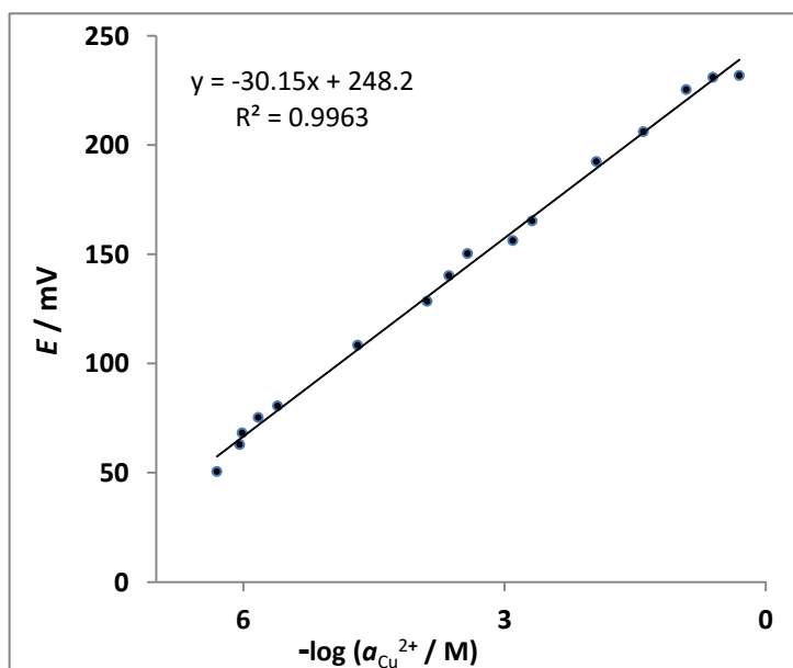
Figure 4. Calibration graph of Cu electrode
