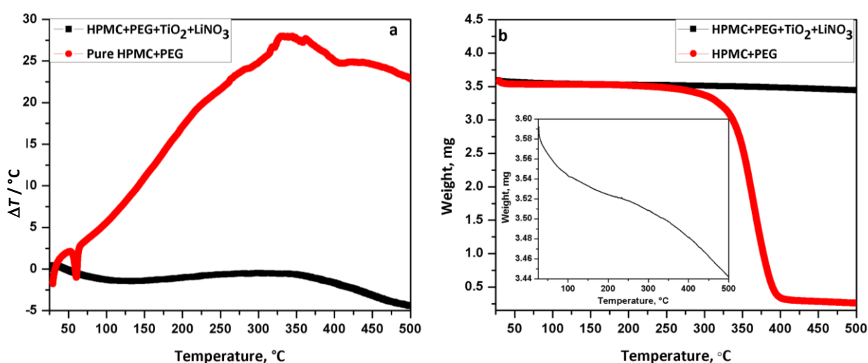
Figure 4. (a) DTA and (b) TGA curves of HPMC/PEG and HPMC/PEG/TiO 2 /LiNO 3 polymer blend electrolytes
