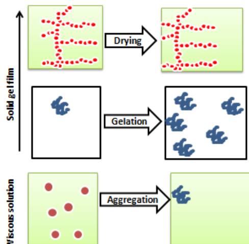
Figure 6. Sol-gel formations
