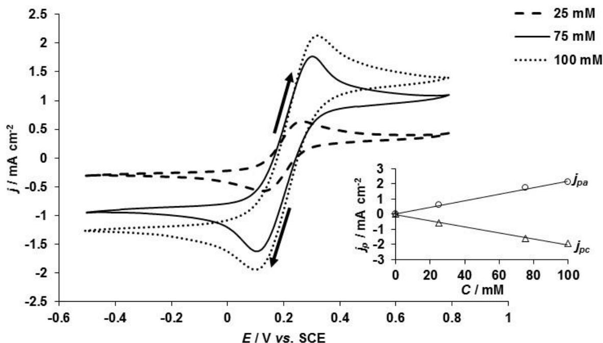
Figure 5 : Cyclic voltammetric curves of ferri/ferrocyanide on boron doped diamond electrode at various redox couple concentration at 480 \text{ mV min}^{-1} , T = 25^\circ\text{C} , CE: Pt, RE: SCE, in the inset : evolution of current peak against redox couple concentration
