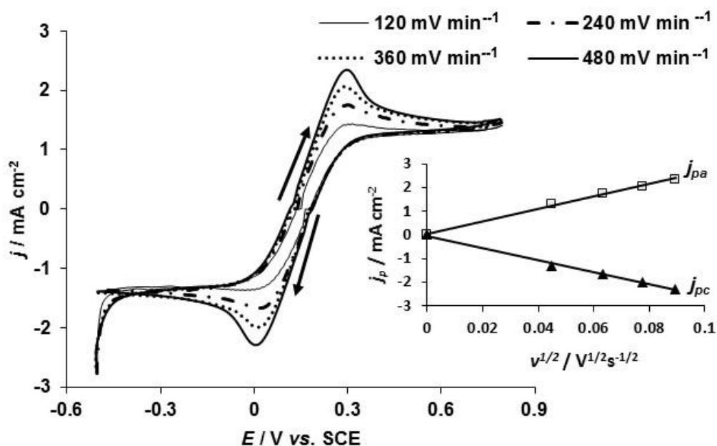
Figure 4 : Cyclic voltammetric curves of ferri/ferrocyanide on boron doped diamond electrode at various potential scan rates ( 120 \text{ mV min}^{-1} - 480 \text{ mV min}^{-1} ), C = 100 \text{ mM} , T = 25^\circ\text{C} , CE: Pt, RE: SCE, in the inset: evolution of current peak against square root of potential scan rates
