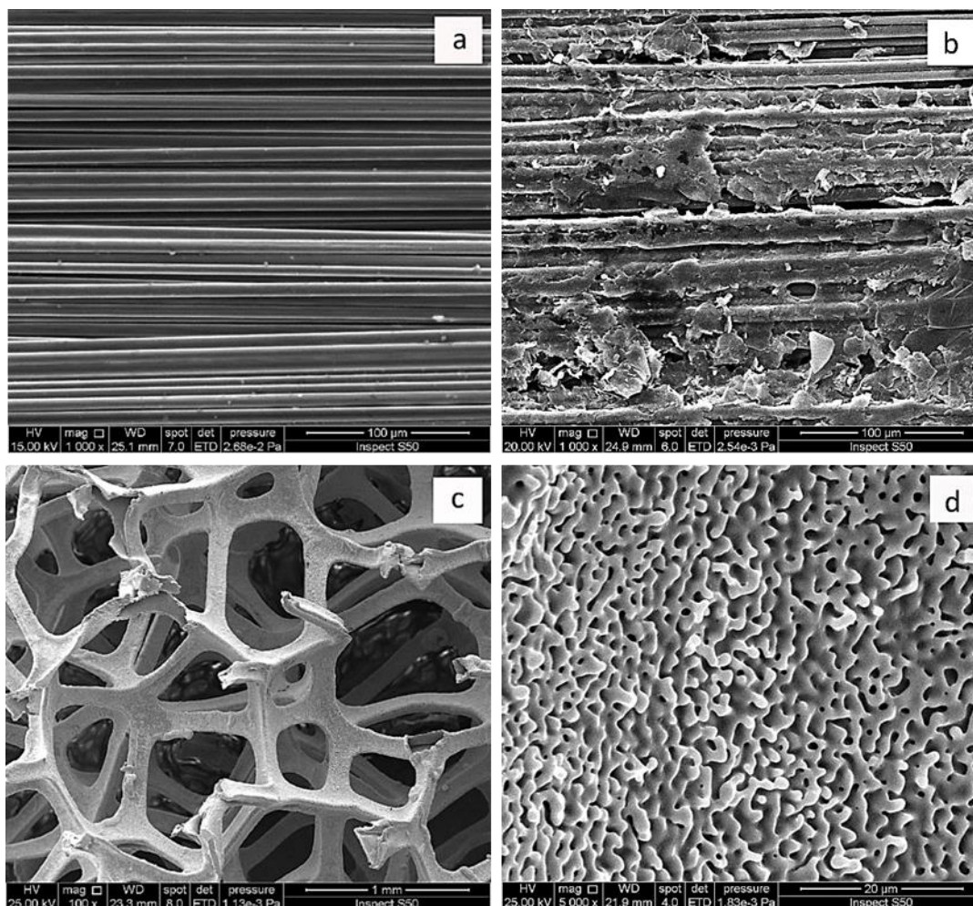
Figure 3. SEM images of: a - CF before modification, b to d - CF after modification with graphene and iron foam before the electro-Fenton process
