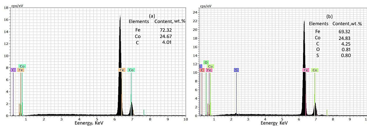
Figure 4. EDX results for iron foam: (a) before reaction, (b) after reaction
