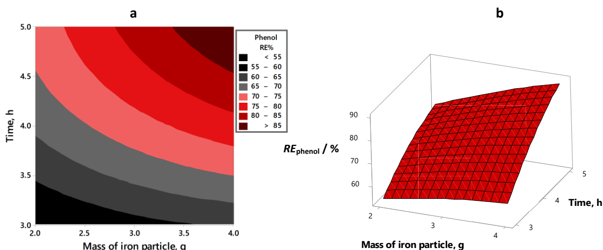
Figure 6. Effect of time and amount of iron particles on RE_{\text{phenol}} at hold value of graphene 0.75 g: (a) contour plot and (b) 3D surface plot
