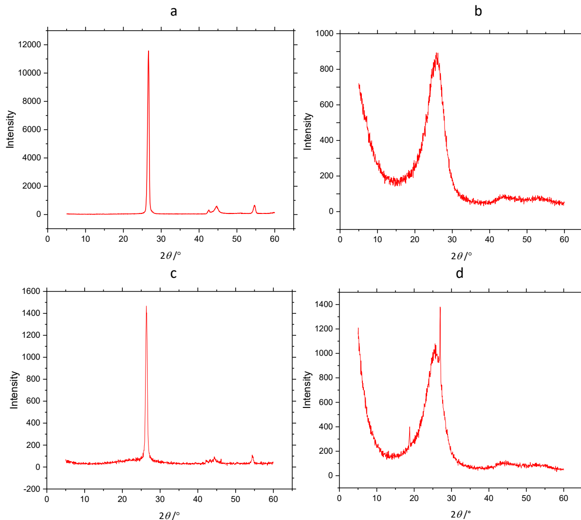
Figure 2. XRD patterns of a - graphite, b - pure CF, c - graphene and d - CF modified with graphene
