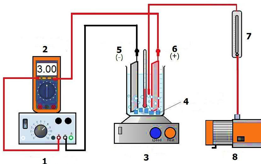
Figure 1. Schematic drawing of the electro-Fenton system: 1) power supply, 2) multimeter, 3) magnetic stirrer, 4) iron particles, 5) cathode, 6) anode, 7) flow meter and 8) pump
