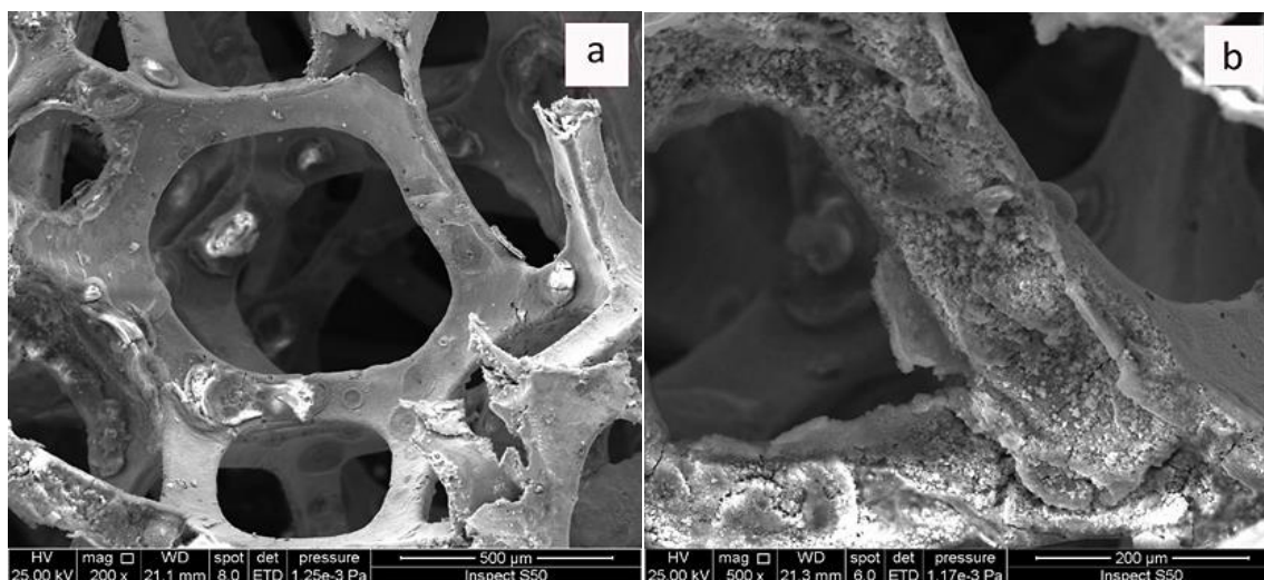
Figure 5. SEM images of iron foam after reaction
