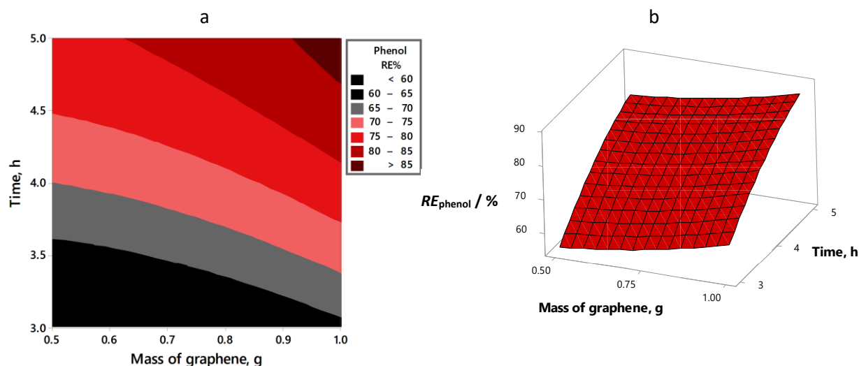
Figure 7. Effect of time and graphene dosage on RE_{phenol} at hold value of iron particles of 3 g: (a) contour plot and (b) 3D surface plot
