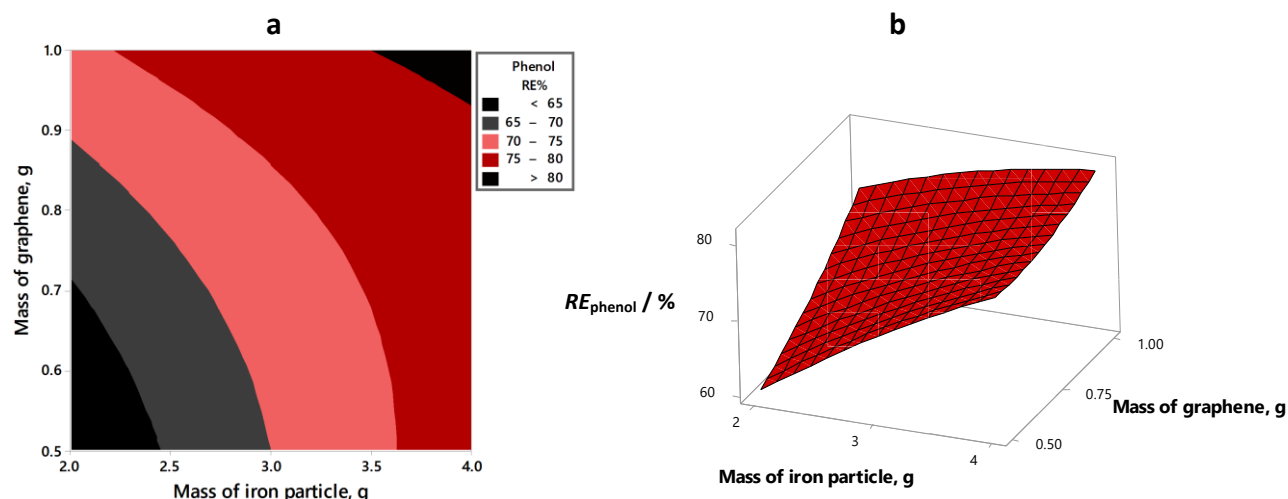
Figure 8. Effect of graphene dosage and amount of iron particles on RE_{phenol} at hold value of time 4h: (a) contour plot, and (b) 3D surface plot
