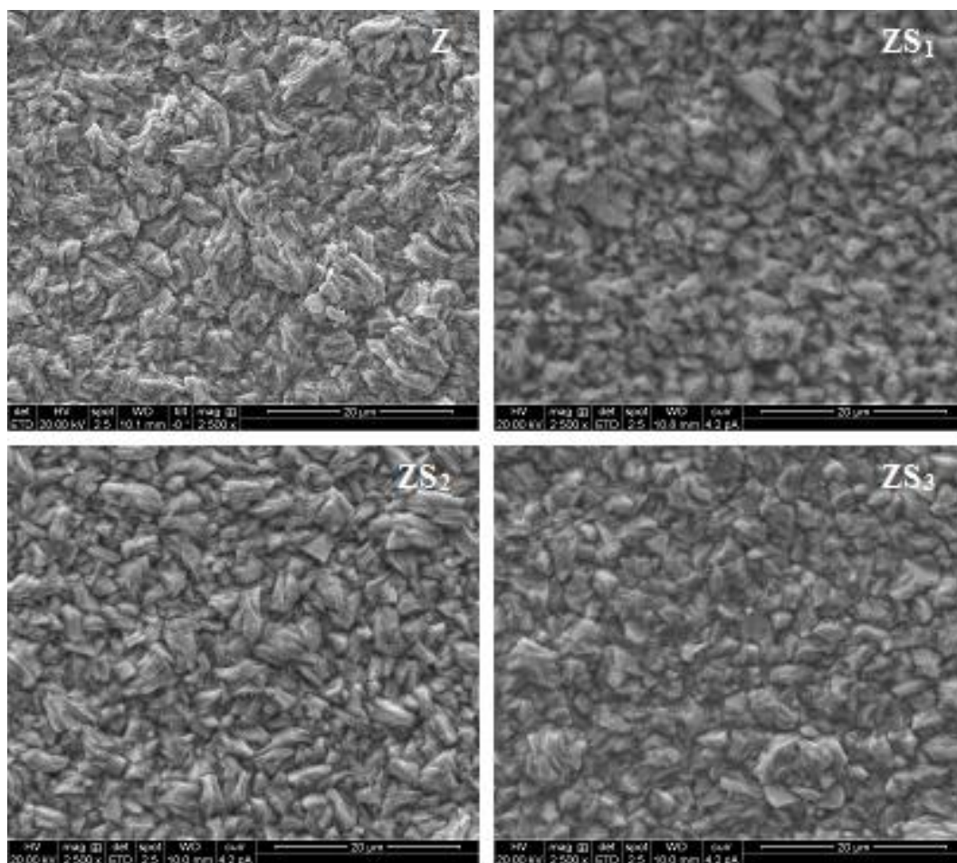
Figure 8. SEM micrographs of zinc and Zn-SiC composite coatings recorded after potentiodynamic polarization measurement.
