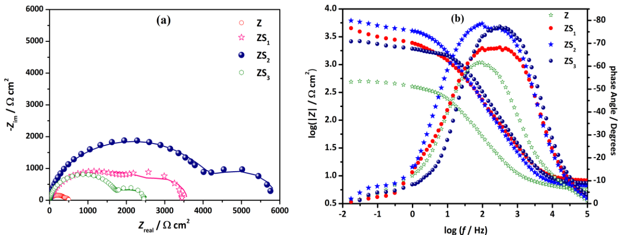
Figure 6. Impedance (a) Nyquist and (b) Bode plots for zinc and Zn-SiC composite coatings measured with respect to Sat. Ag/AgCl electrode in 3.5% NaCl solution.
