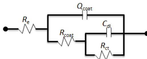
Figure 7. Electrical Equivalent Circuit used to simulate the recorded Impedance Nyquist plots.
