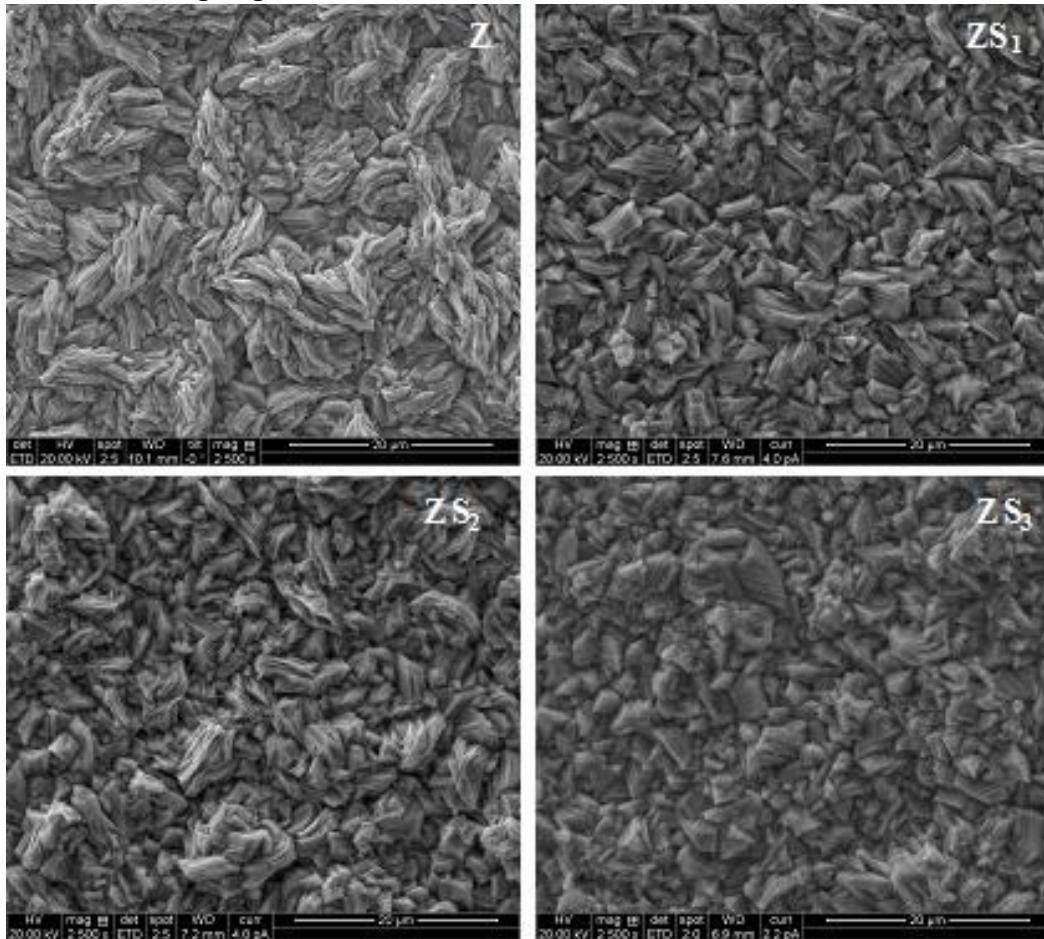
Figure 2. SEM micrographs of as deposited zinc and Zn-SiC composite coatings
