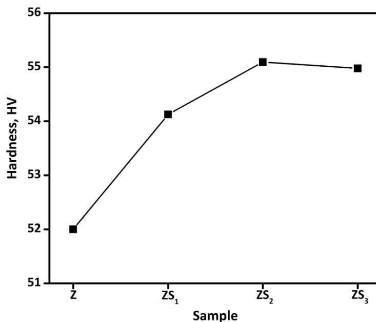
Figure 9. Vickers micro-hardness value of Zn and Zn-SiC MMCs.
