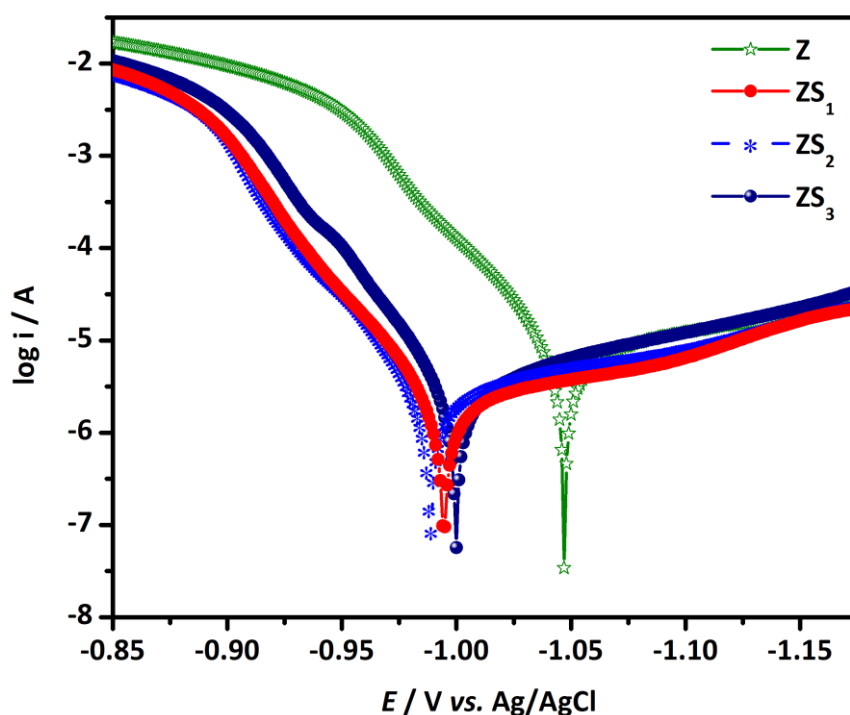
Figure 5. Potentiodynamic polarization curves for zinc and Zn-SiC composite coatings measured with respect to sat. Ag/AgCl electrode in 3.5 % NaCl solution.
