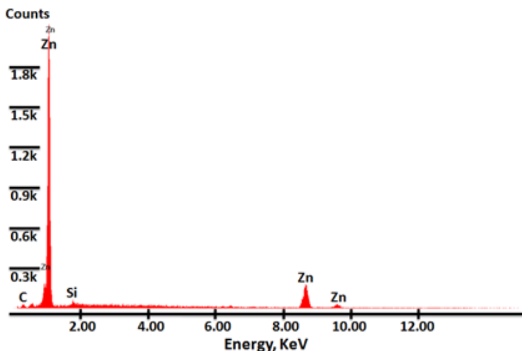
Figure 1. EDX spectra of Zn-SiC composite coating ZS 2
