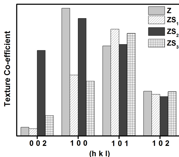
Figure 4. Preferred orientation of crystallites in zinc and Zn-SiC composite coatings.
