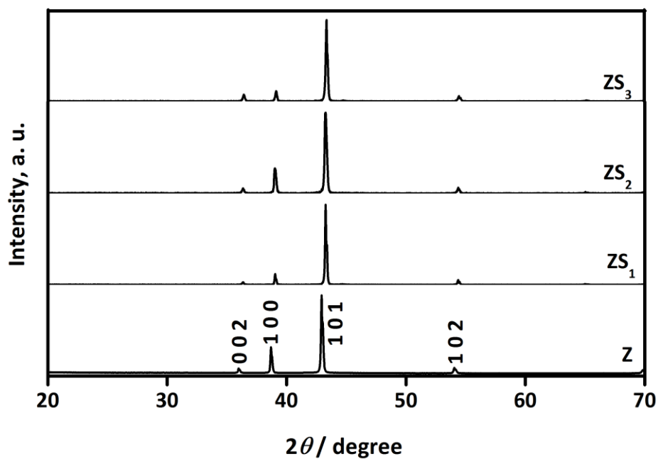
Figure 3. XRD diffractograms obtained from zinc and Zn-SiC composite coatings
