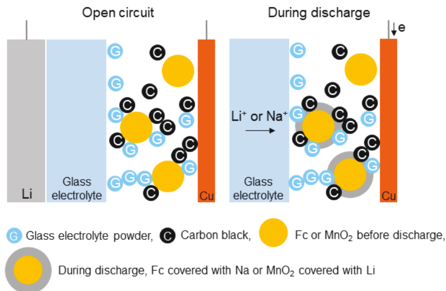
Figure 1. Diagrams of positive electrode active materials reflecting the C[(EC)cC]n mechanism on the Braga-Goodenough Na-Fc and Li-MnO 2 battery under open circuit and discharge conditions
