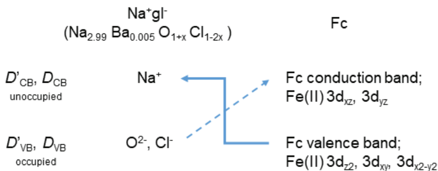
Figure 3. Two possibilities of orbital hybridization in the theory of \phi_{\text{CNL}}^{\text{G}} between Fc and \text{Na}^+\text{gl}^- . The inset arrows show the direction of possible electron transfer at their interfaces. D'_{\text{CB}} and D'_{\text{VB}} respectively correspond to the density of states of the conduction band and valence band of \text{Na}^+\text{gl}^- , and D_{\text{CB}} and D_{\text{VB}} respectively correspond to the density of states of the conduction band and valence band of Fc
