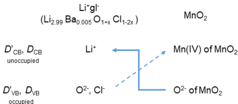
Figure 4. Two possibilities of orbital hybridization in the theory of \phi_{\text{CNL}}^{\text{G}} between \text{MnO}_2 and \text{Li}^+\text{gl}^- . The inset arrows show the direction of possible electron transfer at their interfaces. D'_{\text{CB}} and D'_{\text{VB}} respectively correspond to the density of states of the conduction band and valence band of \text{Li}^+\text{gl}^- , and D_{\text{CB}} and D_{\text{VB}} respectively correspond to the density of states of the conduction band and valence band of \text{MnO}_2
