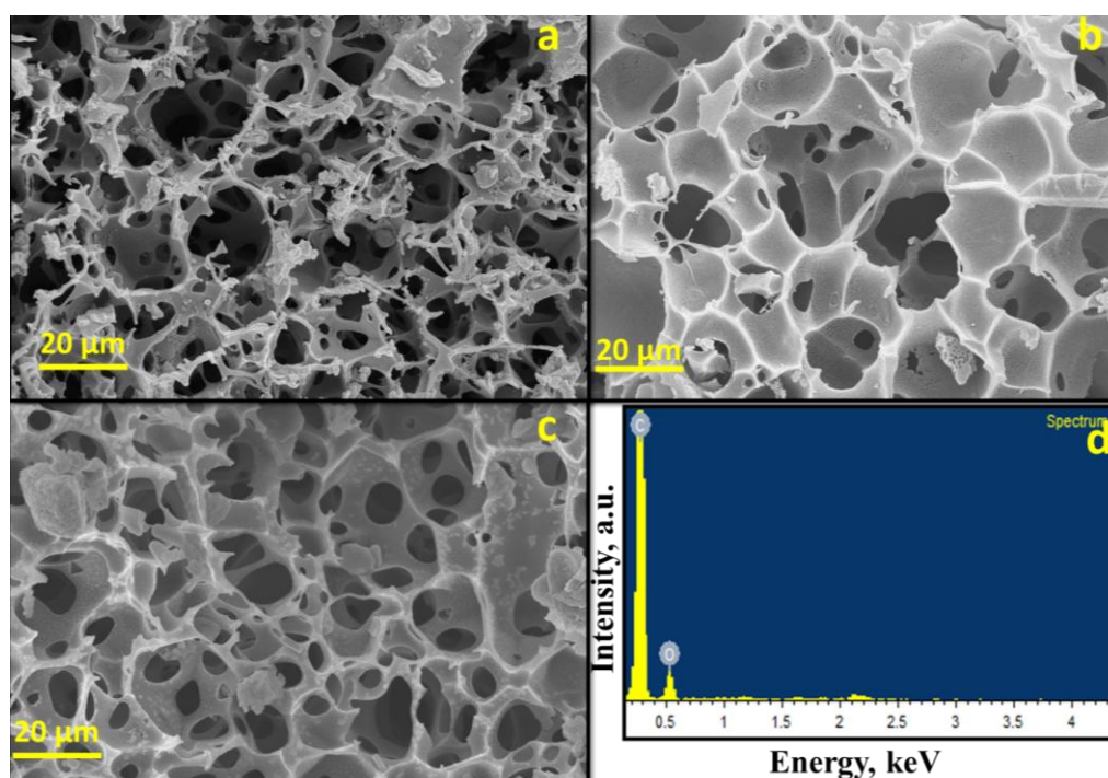
Figure 3. (a-c) SEM images of PPF-700, PPF-800, and PPF-900 based activated carbon at magnification 20,000 x (d) EDAX analysis of PPF-900
