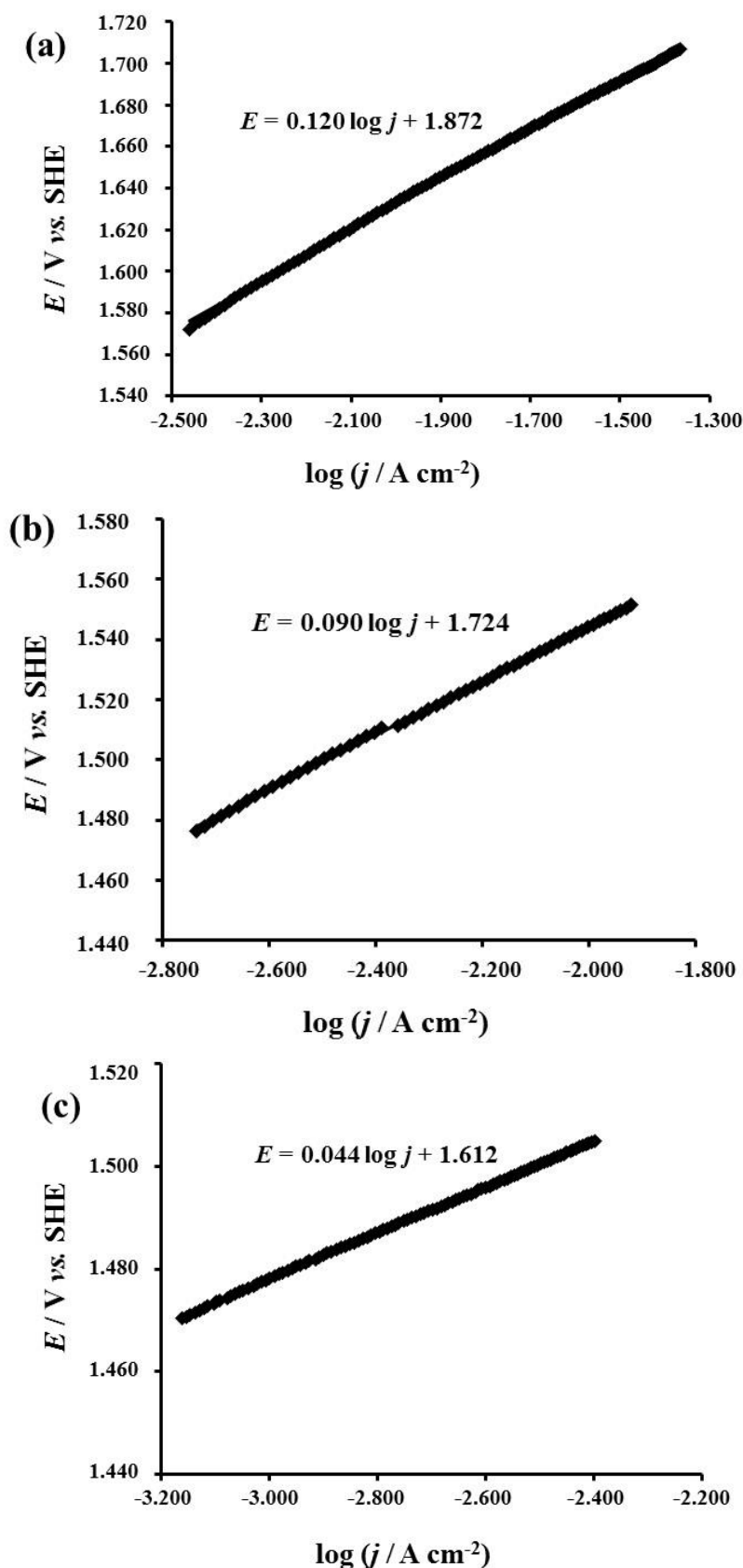
Figure 3 : Tafel line of Pt (a), _{50}\text{Pt}-_{50}\text{RuO}_2 (b) and _{50}\text{Pt}-_{50}\text{IrO}_2 (c) in perchloric acid 1 M ; \nu = 1 \text{ mV s}^{-1} ; CE : platinum; T = 25^\circ\text{C}
