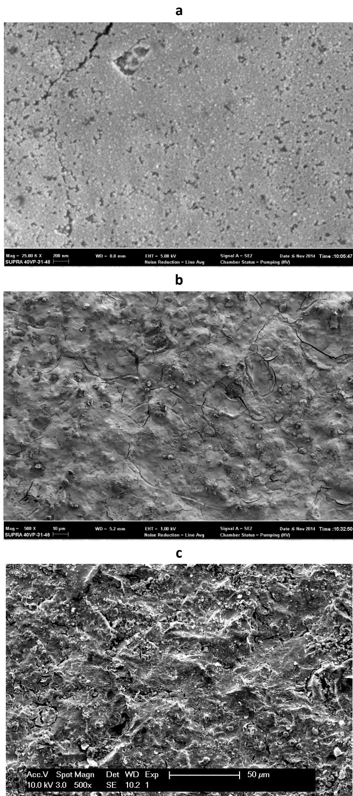
Figure 1: Scanning electron micrographs of Pt( a ), _{50}\text{Pt}-_{50}\text{RuO}_2 ( b ) and _{50}\text{Pt}-_{50}\text{IrO}_2 ( c )
