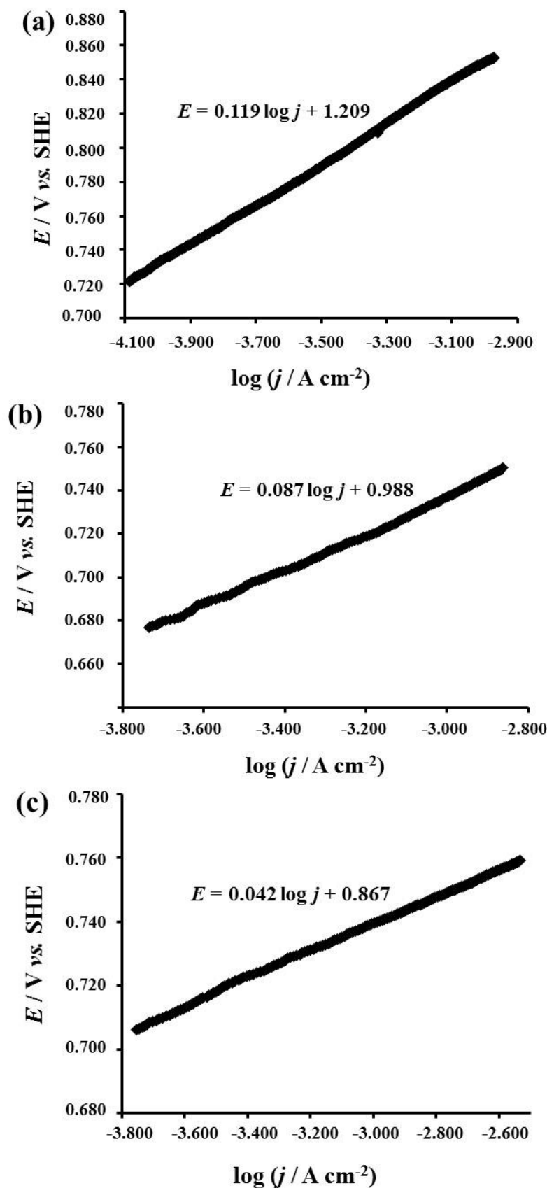
Figure 5. Tafel line of Pt (a), _{50}\text{Pt-}_{50}\text{RuO}_2 (b) and _{50}\text{Pt-}_{50}\text{IrO}_2 (c) in KOH 0.5 M; v = 1 \text{ mV s}^{-1} ; CE : platinum, T = 25^\circ\text{C}
