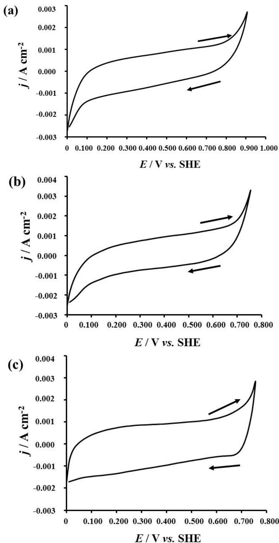
Figure 4. Cyclic voltammograms of Pt (a), 50 Pt- 50 RuO 2 (b) and 50 Pt-50IrO 2 (c) in KOH 0.5 M at 100 mV s -1 , CE : platinum, T= 25°C
