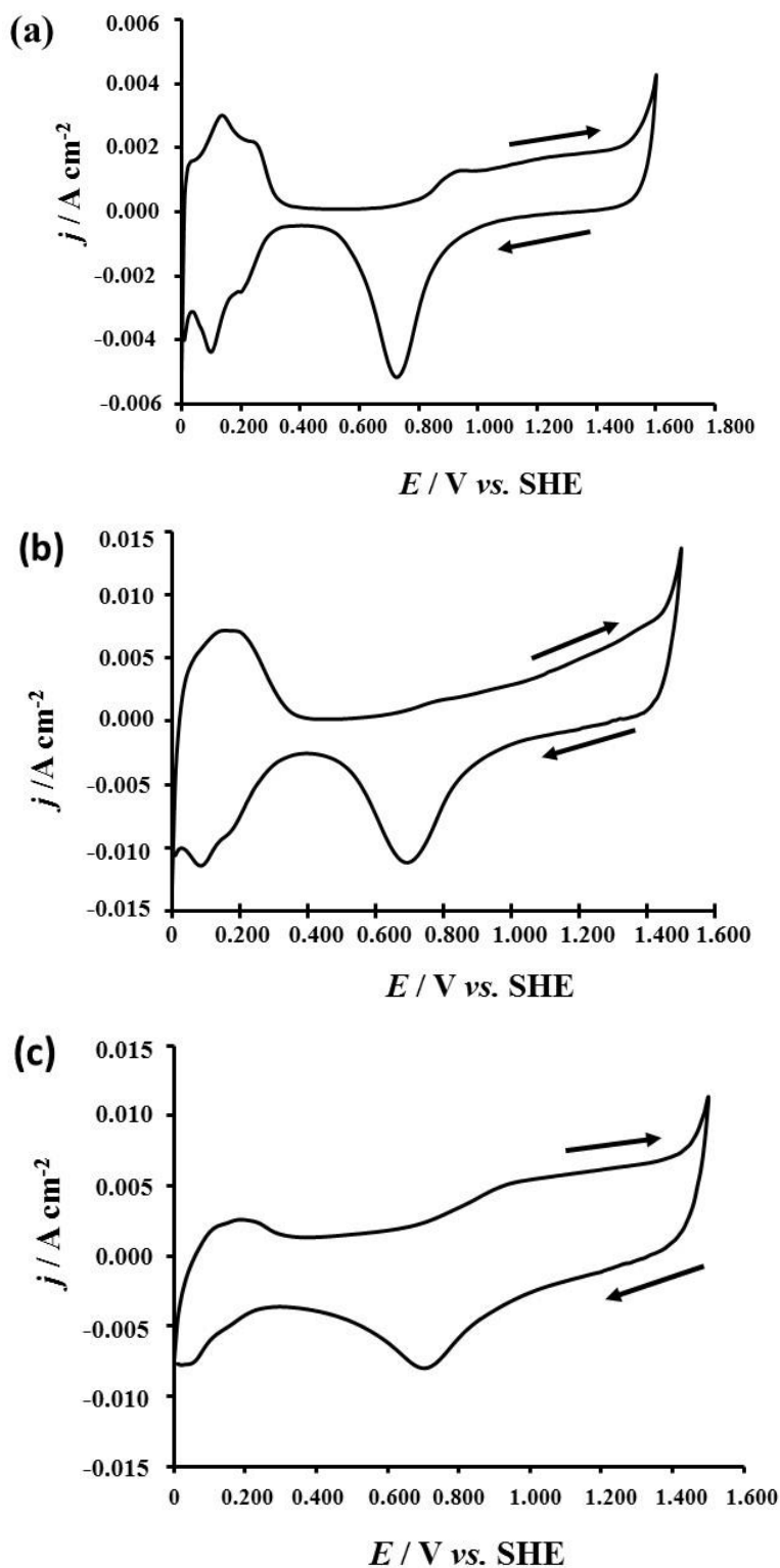
Figure 2: Cyclic voltammograms of Pt (a), _{50}\text{Pt-}_{50}\text{RuO}_2 (b) and _{50}\text{Pt-}_{50}\text{IrO}_2 (c) in 1 M \text{HClO}_4 at 100 \text{ mV s}^{-1} , CE: platinum, T = 25^\circ\text{C}
