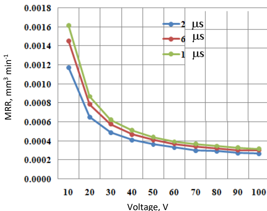
Figure 5. Theoretical variations in MRR with reference to the applied voltage at three different T_{on} / \mu s
