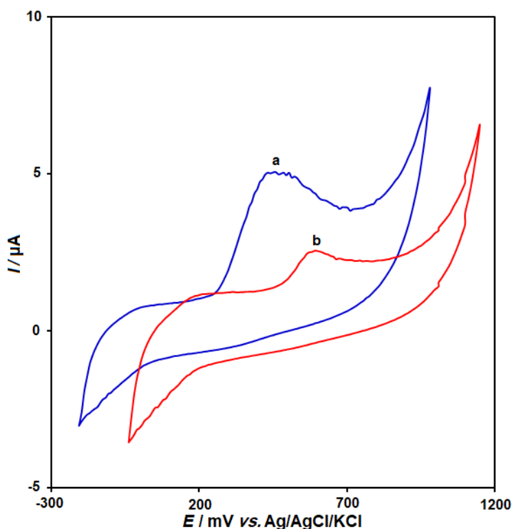
Figure 1. Cyclic voltammograms of (a) Fe_3O_4/GO/GCE and (b) unmodified GCE in 0.1 M PBS (pH 7.0) in the presence of 30.0 \mu M bisphenol A at the scan rate 50\text{ mVs}^{-1}
