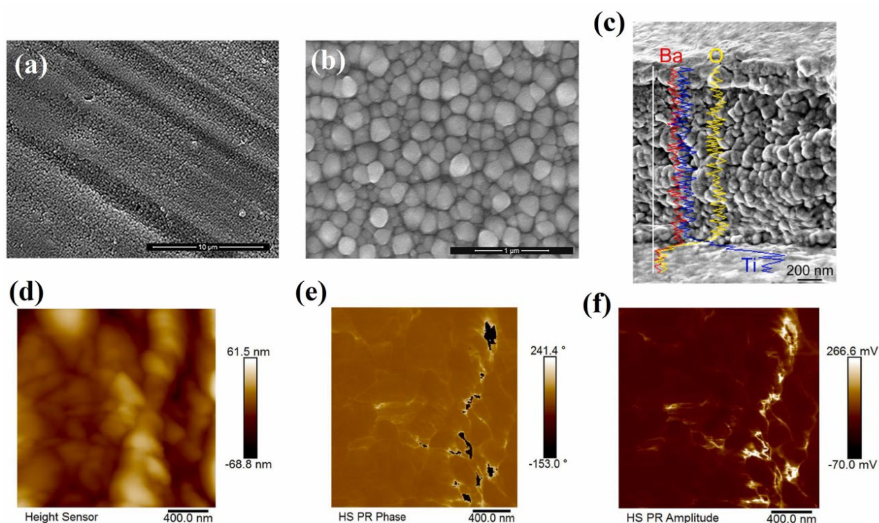
Figure 3. BT coating characteristics. (a, b) Surface SEM images of BT/TC4 materials. (c) Cross-section SEM-EDS picture of BT/TC4 material. (d) AFM topography. (e) PFM phase. (f) PFM amplitude [79]. Permissions under Attribution 4.0 International (CC BY 4.0)
