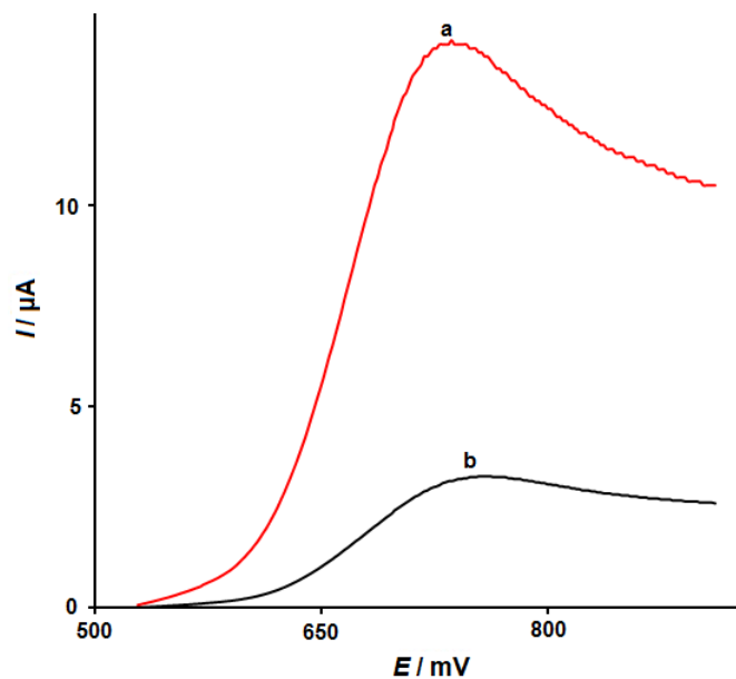
Figure 2. Linear sweep voltammograms of (a) FL-MoS 2 /SPE and (b) bare SPE in 0.1 M PBS (pH 7.0) in the presence of 100.0 \mu\text{M} sunset yellow at the scan rate 50 \text{ mVs}^{-1}
