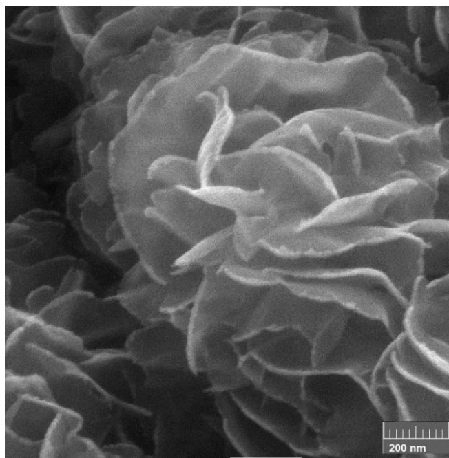
Figure 1. SEM image of flower-like MoS 2
