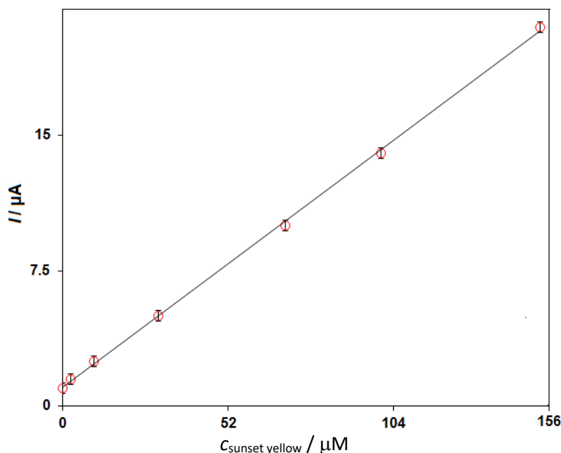
Figure 8. Plot of the electrocatalytic peak current as a function of sunset yellow concentration in the range of 0.1-150.0 \mu\text{M}
