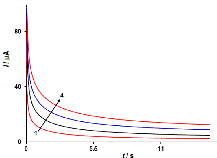
Figure 5. Chronoamperograms obtained at FL-MoS 2 /SPE in 0.1 M PBS (pH 7.0) for different concentration of sunset yellow. Numbers 1-4 correspond to 0.1, 0.75, 1.1 and 1.5 mM of sunset yellow
