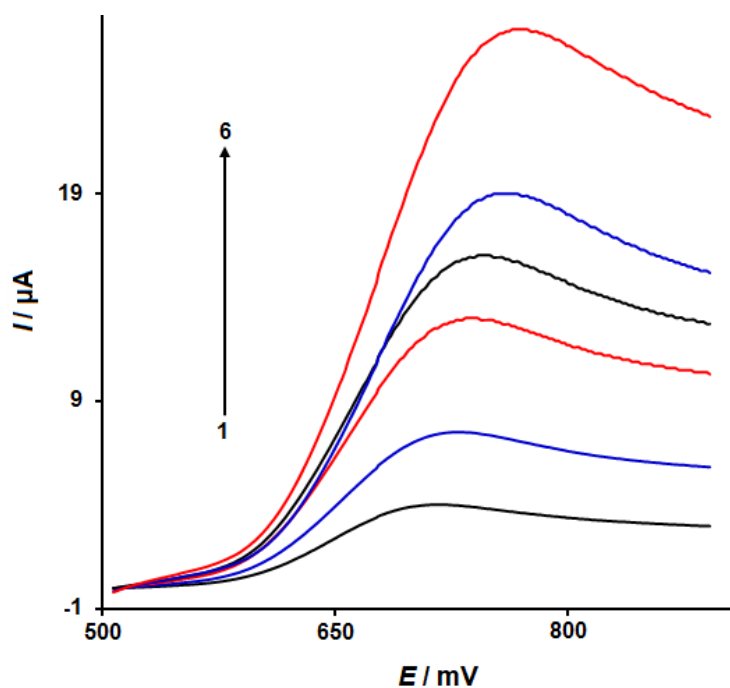
Figure 3. Linear sweep voltammograms of FL-MoS 2 /SPE in 0.1 M PBS (pH 7.0) containing 50.0 \mu\text{M} sunset yellow at various scan rates; 1-6 correspond to 5, 15, 45, 70, 100 and 200 \text{mVs}^{-1} , respectively
