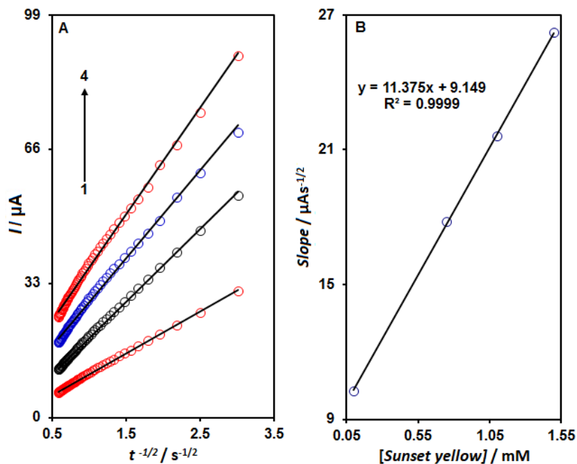
Figure 6. (A) Plots of I vs. t^{-1/2} obtained from chronoamperograms 1-4, (B) plot of the slope of the straight lines against sunset yellow concentration (0.1-1.5 mM)
