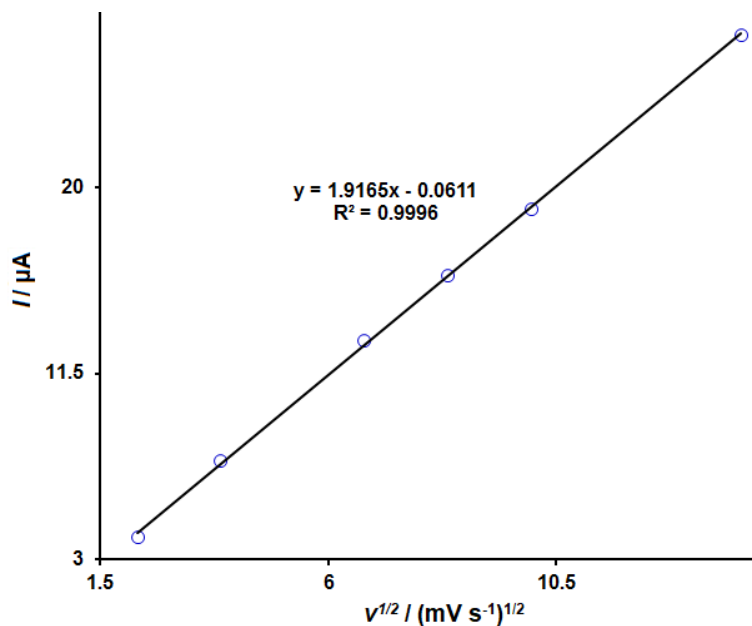
Figure 4. Plot of anodic peak current vs. v^{1/2} at different scan rates in the range of 5 to 200 mV/s.
