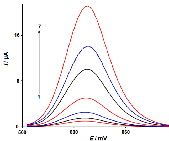
Figure 7. DPVs of FL-MoS 2 /SPE in 0.1 M (pH 7.0) containing different concentrations of sunset yellow. Numbers 1–7 correspond to 0.1, 2.5, 10.0, 30.0, 70.0, 100.0 and 150.0 μM of sunset yellow
