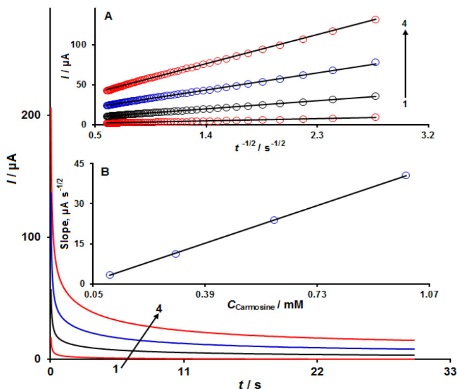
Figure 5. Chronoamperograms obtained at g-C 3 N 4 /ILs/CPE in 0.1 M PBS (pH 7.0) for different concentration of carmoisine. The 1-4 correspond to 0.1, 0.3, 0.6 and 1.0 mM of carmoisine. Insets: (A) Plots of I vs. t^{-1/2} obtained from chronoamperograms 1-4. (B) A plot of the slope of the straight lines against carmoisine concentration
