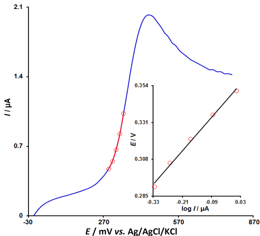
Figure 4. Tafel plot for g\text{-C}_3\text{N}_4/\text{ILs}/\text{CPE} in 0.1\text{ M PBS (pH 7.0)} in the presence of 35.0\ \mu\text{M} carmoisine and scan rate 10\ \text{mV s}^{-1}
