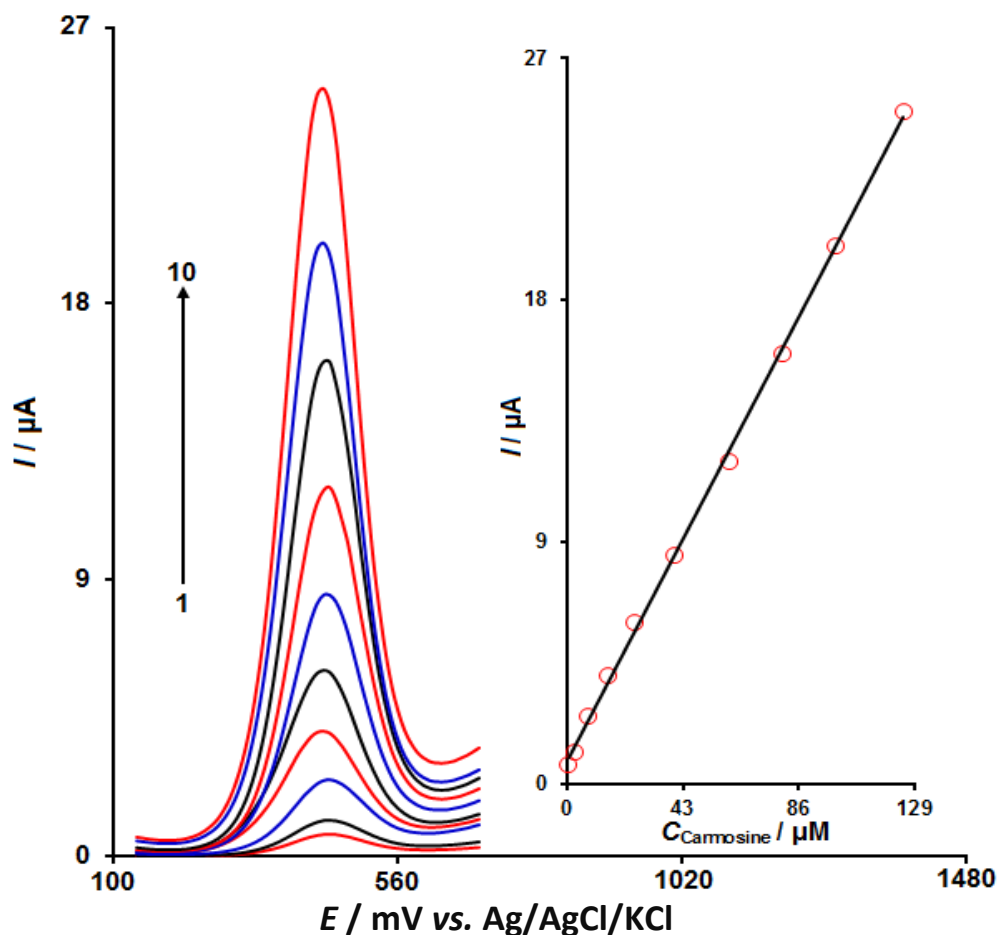
Figure 6. DPVs of g\text{-C}_3\text{N}_4/\text{ILs}/\text{CPE} in 0.1 M (pH 7.0) containing different concentrations of carmoisine. Numbers 1–10 correspond to 0.4, 2.5, 7.5, 15.0, 25.0, 40.0, 60.0, 80.0, 100.0 and 125.0 \mu\text{M} of carmoisine. Inset: plot of the electrocatalytic peak current as a function of carmoisine concentration in the range of 0.4–125.0 \mu\text{M}
