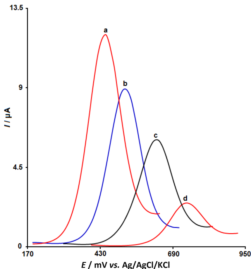
Figure 2. Differential pulse voltammograms of (a) g-C 3 N 4 /ILs/CPE, (b) g-C 3 N 4 /CPE, (c) ILs/CPE and (d) bare CPE in 0.1 M PBS (pH 7.0) in the presence of 60.0 μM carmoisine at the scan rate 50 mV s -1
