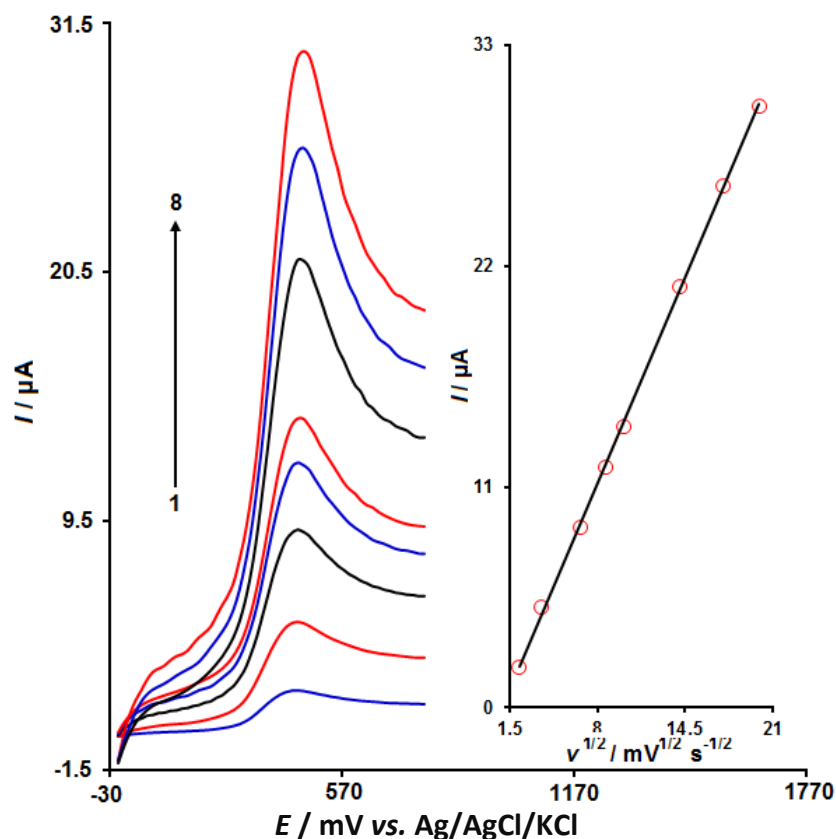
Figure 3. Linear sweep voltammograms of g\text{-C}_3\text{N}_4/\text{ILs}/\text{CPE} in 0.1\text{ M PBS (pH 7.0)} containing 35.0\ \mu\text{M} carmoisine at various scan rates; 1-8 correspond to 5, 15, 45, 75, 100, 200, 300 and 400\ \text{mV s}^{-1} , respectively. Inset: variation of anodic peak current vs. v^{1/2}
