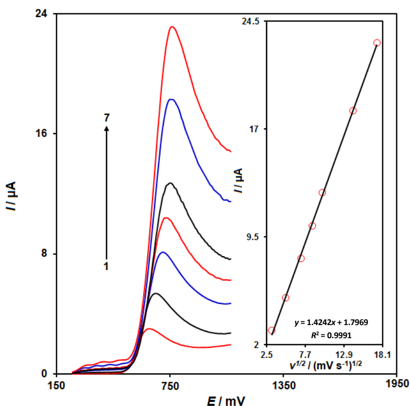
Figure 5. Linear sweep voltammograms of V_2O_5 -NP/SPE in 0.1 \text{ M PBS} (pH 7.0) containing 80.0 \mu\text{M} amaranth at various scan rates; 1-7 correspond to 10, 25, 50, 75, 100, 200 and 300 \text{ mV s}^{-1} , respectively. Inset: variation of anodic peak current vs. \nu^{1/2}
