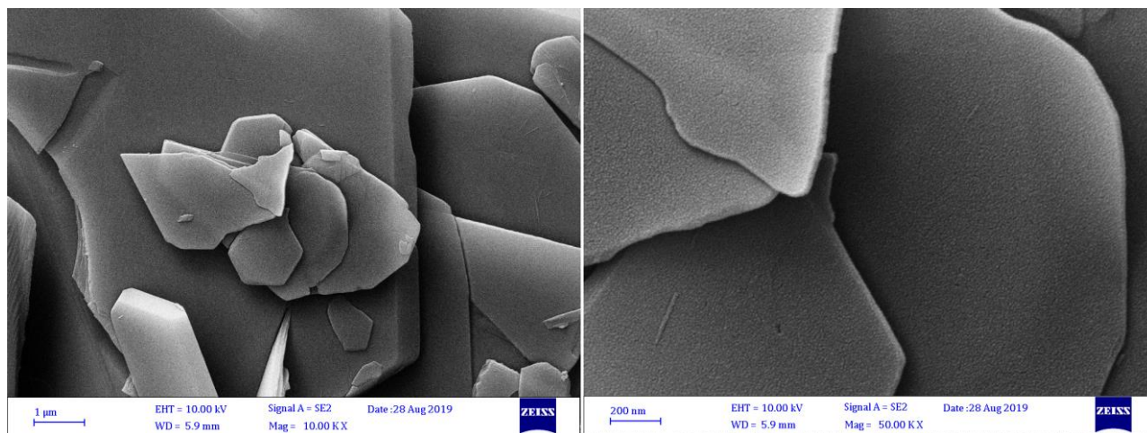
Figure 1. The FE-SEM images of V_2O_5 nanoplates at different magnifications
