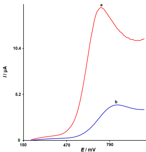
Figure 4. Linear sweep voltammograms curves of unmodified SPE (curve b) and V_2O_5 -NP/SPE (curve a) in 0.1 M PBS containing 80.0 \mu\text{M} amaranth; scan rate: 50 \text{mV s}^{-1}
