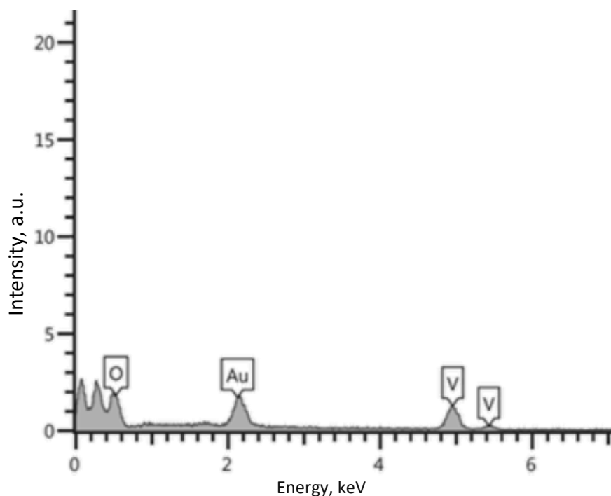
Figure 2. The EDX spectrum of V_2O_5 nanoplates
