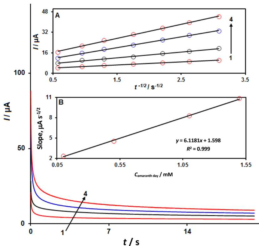
Figure 6. Chronoamperograms obtained at V 2 O 5 -NP/SPE in 0.1 M PBS at pH of 7.0 for different concentrations of amaranth (1-4 refer to: 0.1, 0.5, 1.1 and 1.5 mM). A - The I plot versus t -1/2 observed by chronoamperograms 1-4; B - The slope plot of the straight line vs. concentration of amaranth
