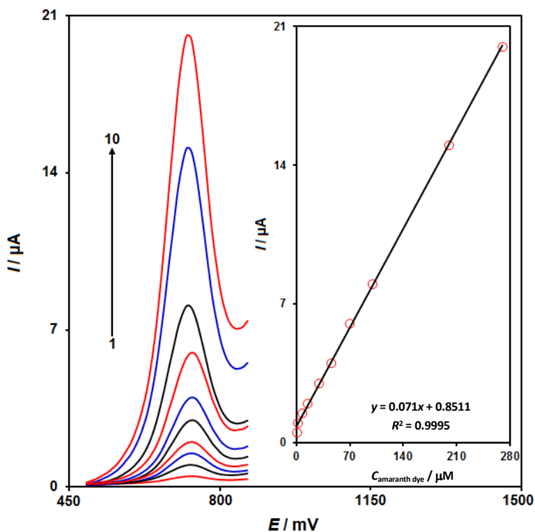
Figure 7. DPVs of V 2 O 5 -NP/SPE in 0.1 M (pH 7.0) containing different concentrations of amaranth. Numbers 1–10 correspond to to 0.1, 2.0, 7.0, 15.0, 30.0, 45.0, 70.0, 100.0, 200.0 and 270.0 µM of amaranth. Inset: plot of the electrocatalytic peak current as a function of amaranth concentration in the range of 0.1-270.0 µM
