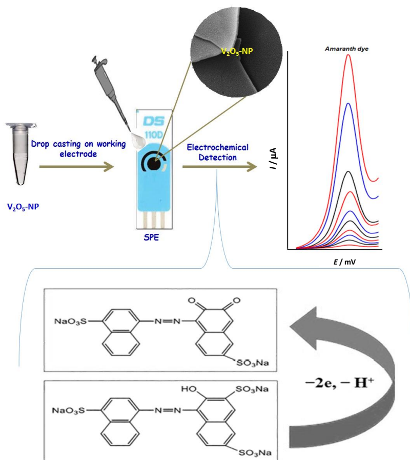
Scheme 1. The schematic preparation of V 2 O 5 -NP/SPE for determination of amaranth
