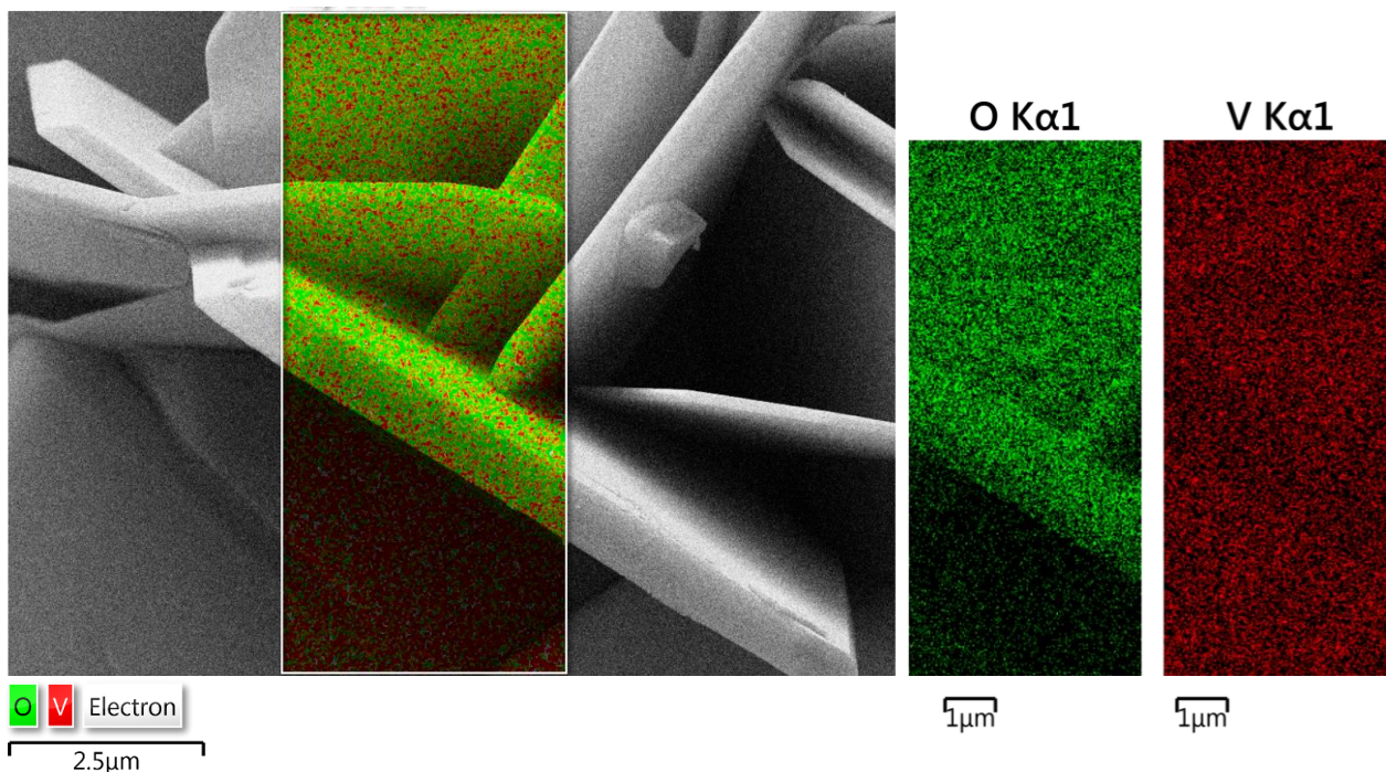
Figure 3. The elemental mapping images of V_2O_5 nanoplates
