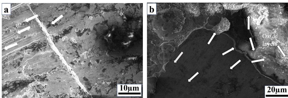
Figure 11. SEM images of worn surface of Coating-1 heat treated at: (a) 400°C, 1h; (b) 600°C, 1h.
