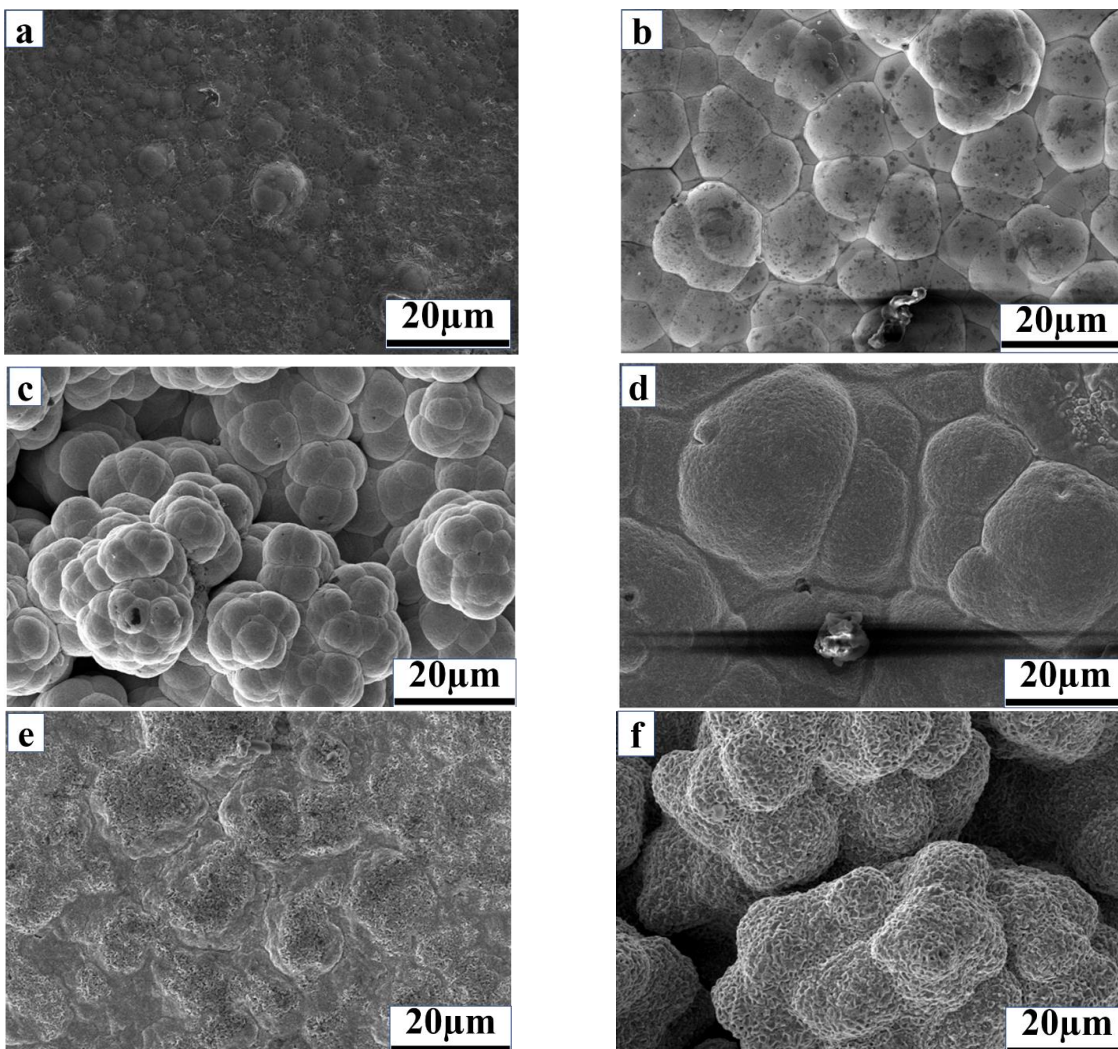
Figure 2. FESEM images of Coating-2: (a) as-deposited; (b) heat treated at 400 °C, 1 h; (c) heat treated at 400 °C, 4 h; (d) heat treated at 600 °C, 1 h; (e) heat treated at 600 °C, 4 h; (f) heat treated at 800 °C, 1 h
