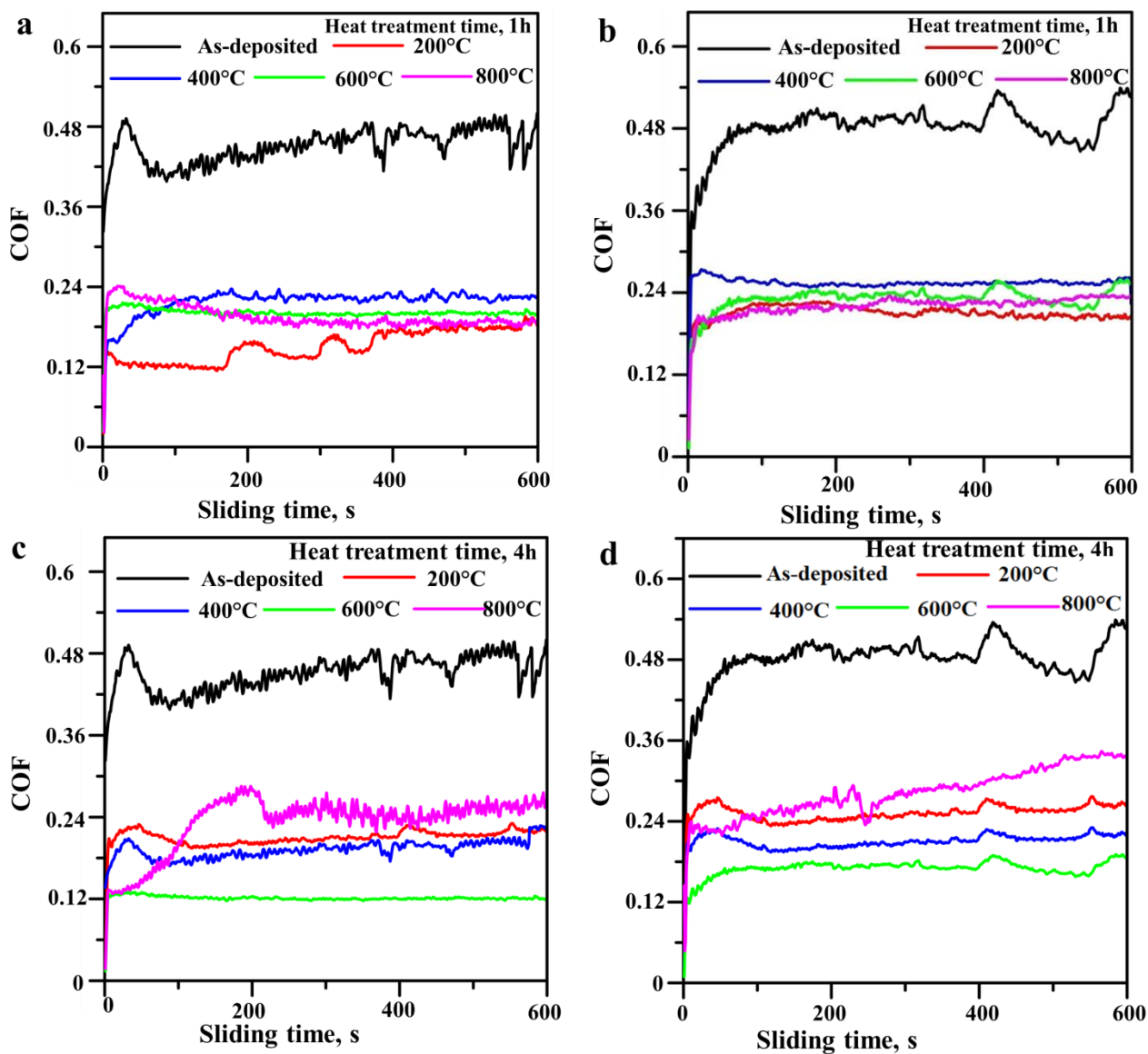
Figure 8. COF vs. sliding duration plots of: (a) Coating-1, 1 h; (b) Coating-2, 1 h; (c) Coating-1, 4 h; (d) Coating-2, 4 h
