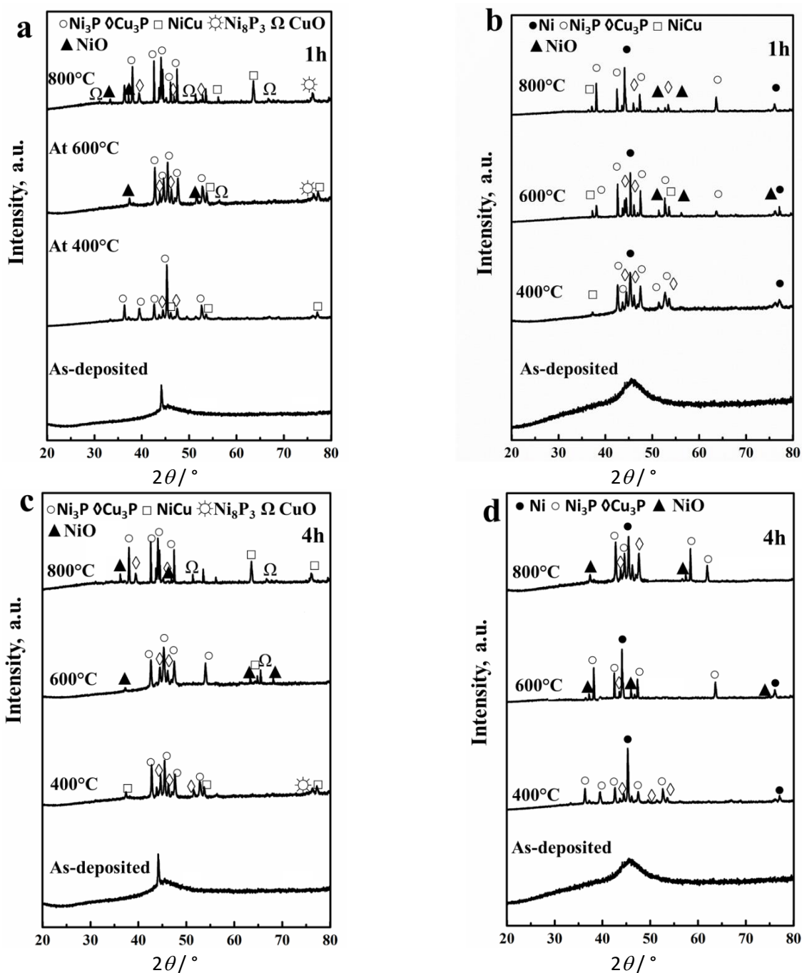
Figure 5. XRD plots of: (a) Coating-1, 1 h; (b) Coating-2, 1 h; (c) Coating-1, 4 h; (d) Coating-2, 4 h
