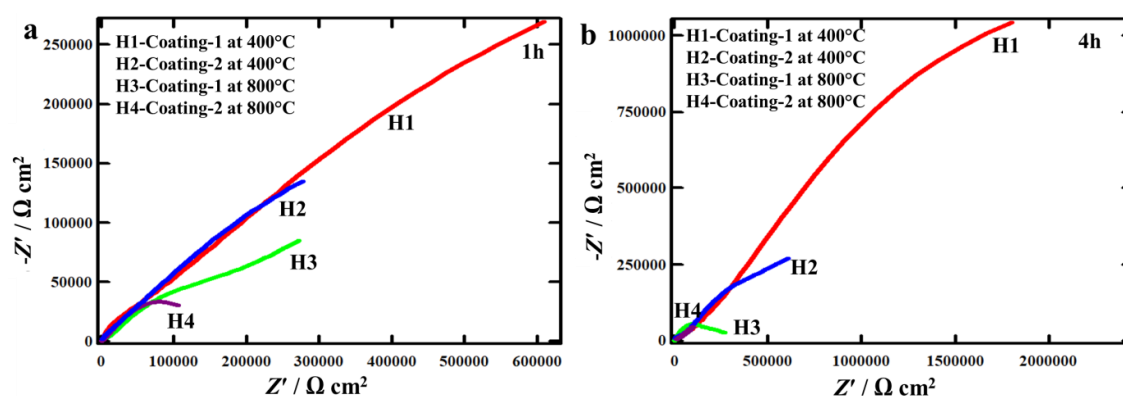
Figure 17. Nyquist plots for heat-treated samples: (a) 1 h duration; (b) 4 h duration
