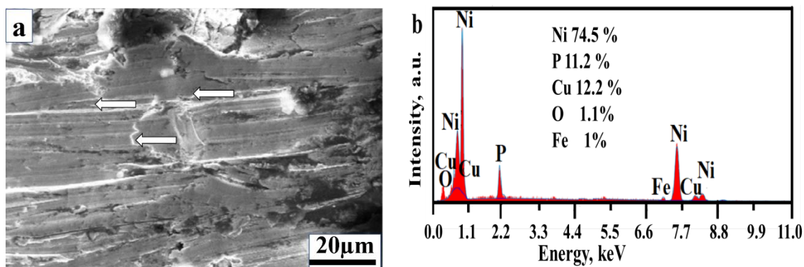
Figure 10. Worn surface of as-deposited Coating-1: (a) SEM image; (b) EDX plot
