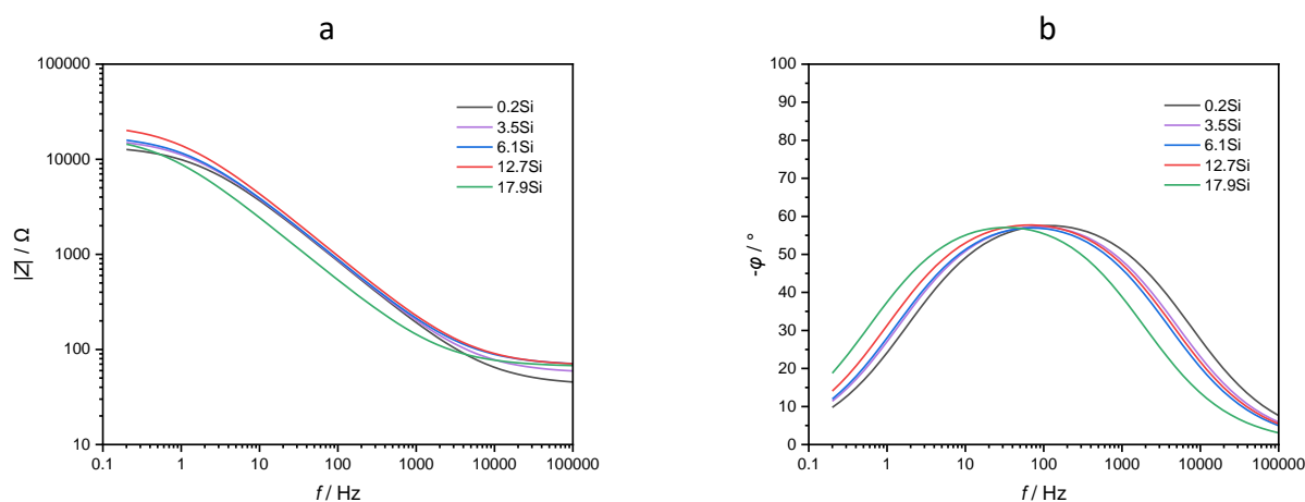
Figure 3. Bode plots for experimental alloys: (a) Bode magnitude plots ( |Z| vs. frequency), (b) Bode phase plot (phase angle vs. frequency)
