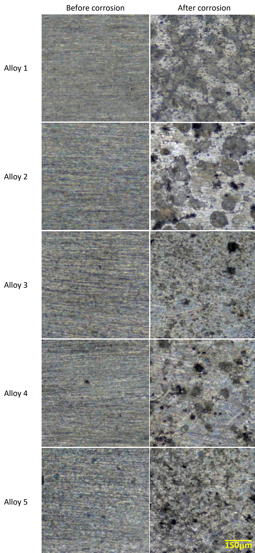
Figure 5. Microstructure of polished Al-Si alloys before and after corrosion in 0.1 M NaCl solution
