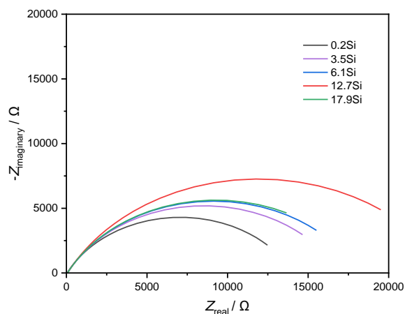
Figure 2. Nyquist plots for experimental automotive alloys in 0.1 M NaCl solution at room temperature
