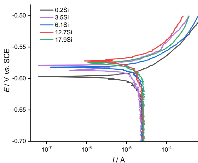
Figure 4. Potentiodynamic polarization curves of automotive Al-Si alloys with varying levels of Si tested in 0.1 M NaCl
