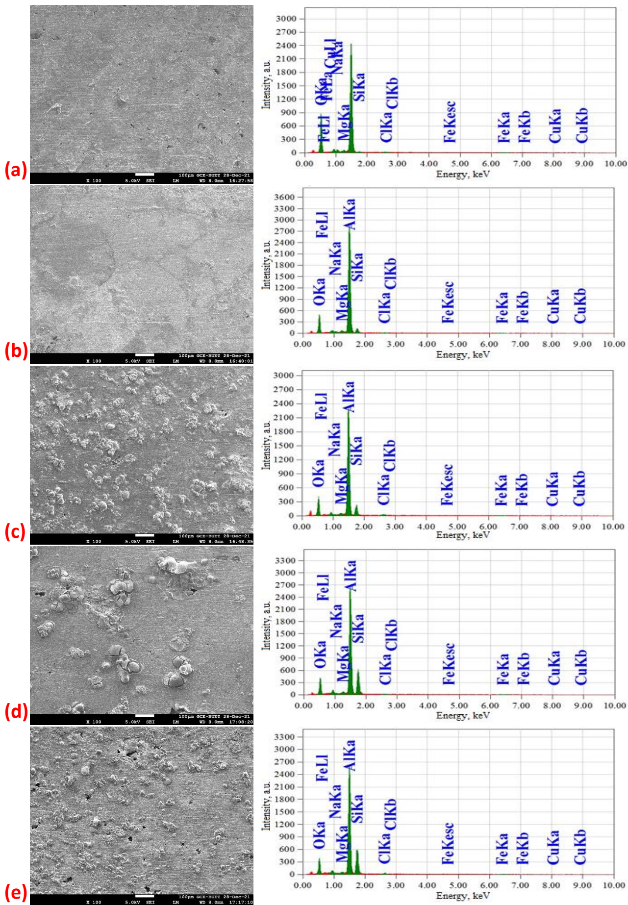
Figure 6. SEM images and EDX spectra of Al-Si alloys after exposure to 0.1 M NaCl solution: (a) 0.2Si, (b) 3.5Si, (c) 6.1Si, (d) 12.7Si, (e) 17.9Si
