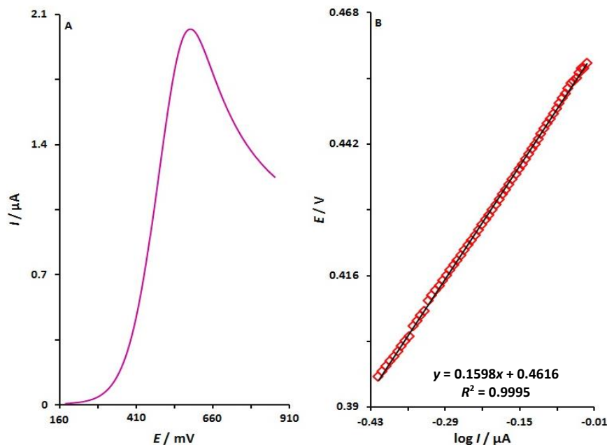
Figure 4. A) LSV response for 100.0 \mu\text{M} folic acid with 10 \text{ mVs}^{-1} scan rate; B) Tafel plot derived from the rising part of the corresponding voltammogram
