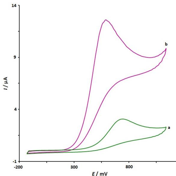
Figure 2. CV curves of unmodified SPE (curve a) and Ni-BTC MOF/SPE (curve b) in 0.1 M PBS containing 200.0 μM folic acid; scan rate: 50 mV s -1 .
