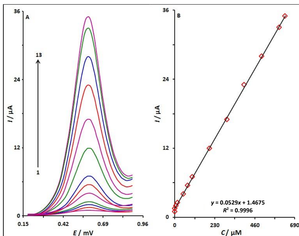
Figure 6. DPV responses of folic acid on Ni-BTC MOF/SPE at different folic acid concentrations (1-13 refer to: 0.08, 1.0, 7.5, 15.0, 50.0, 75.0, 100.0, 200.0, 300.0, 400.0, 500.0, 600.0, and 635.0 \mu\text{M} ) in 0.1 M PBS (pH 7.0). Inset: The relationship between the oxidation peak currents and folic acid concentration
