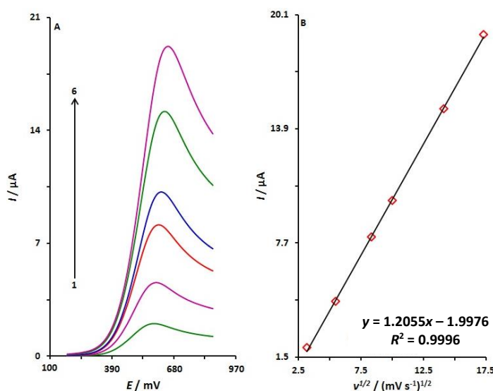
Figure 3. A) LSV curves of 100.0 μM folic acid in 0.1 M PBS (pH 7.0) at a scan rate of 10 to 300 mV s -1 at Ni-BTC MOF/SPE (1-6 refers to 10, 30, 70, 100, 200, and 300 mV s -1 ). B) Plot of the square root of the scan rate vs. the oxidation peak current of folic acid
