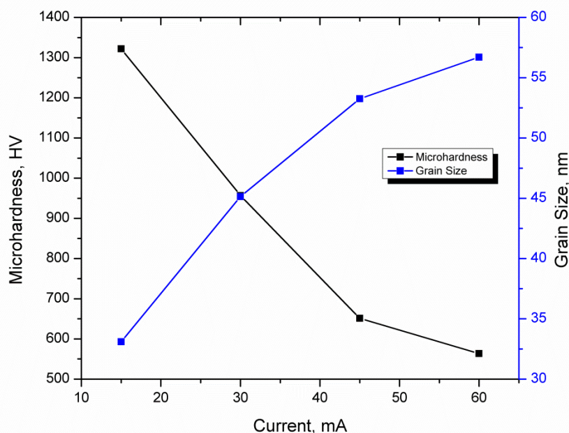
Figure 4. Effect of current on microhardness and grain size of composite layer at pH 3.5 and temperature of 30 °C.
