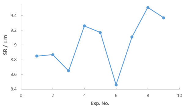
Figure 4. Surface roughness of IN718 versus experiment number
