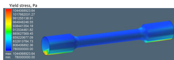
Figure 14. The contour map showing the yield stress simulation result at 375 W
