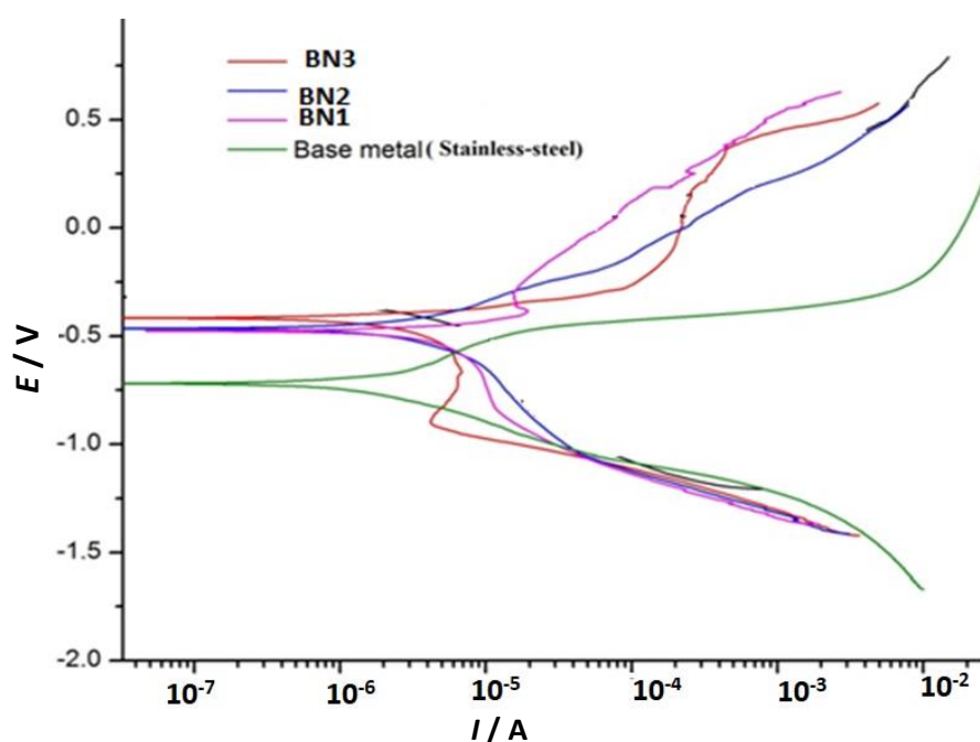
Figure 9. Tafel plots of different boron nitride based coatings
