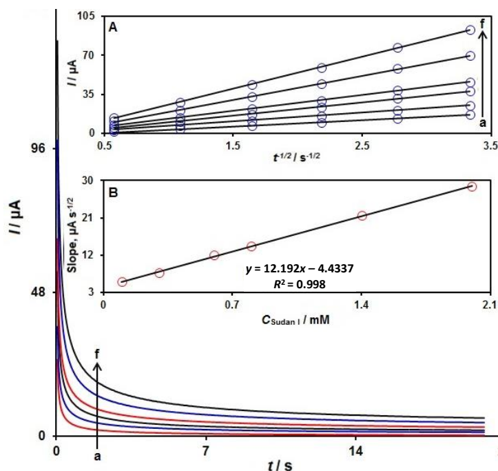
Figure 5. The chronoamperograms obtained on Fe_3O_4 -ZIF-67/ILCPE in PBS (0.1 M, pH 7.0) at different Sudan I concentrations; Note a–f : 0.1, 0.3, 0.6, 0.8, 1.4, and 2.0 mM of Sudan I. Inset A) plot of I versus t^{-1/2} based on chronoamperograms (a – f). Inset B) slope plot of straight line versus Sudan I concentration
