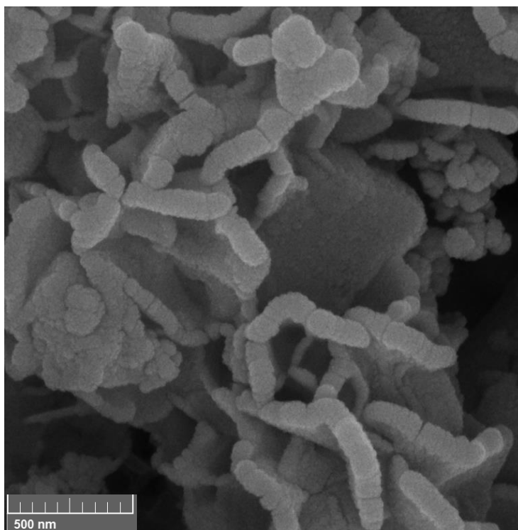
Figure 1. The FE-SEM image of Fe 3 O 4 -ZIF-67 nanocomposite
