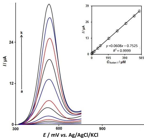
Figure 6. DPV response of Sudan I at Fe_3O_4 -ZIF-67/ILCPE in the concentration range 0.5 - 560.0 \mu M in PBS (0.1 M, pH 7.0); a–k refers to 0.5, 2.5, 10.0, 30.0, 70.0, 100.0, 200.0, 300.0, 400.0, 500.0, and 560.0 \mu M; inset: The calibration curve of DPV peaks against concentration of Sudan I
