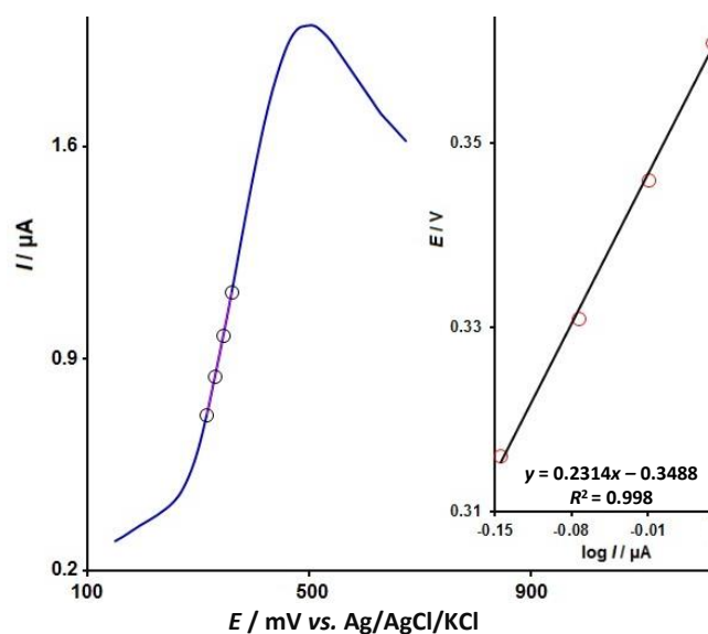
Figure 4. LSV response for 100.0 \mu\text{M} of Sudan I at the scan rate of 10 mV/s; inset: Tafel plot of rising sector or related voltammogram
