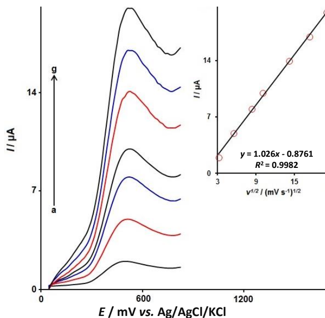
Figure 3. LSV curves of 100.0 \mu\text{M} Sudan I in PBS (0.1 M, pH 7.0) at different scan rates (10–400 mV/s) on \text{Fe}_3\text{O}_4\text{-ZIF-67/ILCPE} (a–g refers to 10, 30, 70, 100, 200.0, 300.0, and 400.0 mV/s). Inset: Plot of scan rate square root versus Sudan I oxidation peak current
