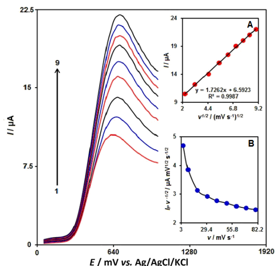
Figure 3. Linear sweep voltammograms of GQDs/2CBF/IL/CPE in 0.1 M PBS, pH 7.0 with 100.0 μM levodopa, at distinct scan rates (1-9 correspond to 5, 10, 20, 30, 40, 50, 60, 70, and 80 mV s -1 ). Insets: (A) variation of anodic peak current with v 1/2 ; (B) variation of scan rate normalized currents (I p /v 1/2 ) with scan rate
