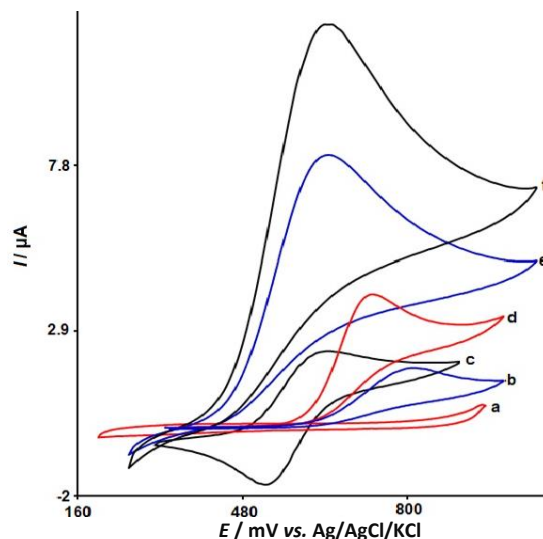
Figure 2. CVs ( 10 \text{ mVs}^{-1} ) of unmodified and modified CPEs in 0.1M PBS (pH 7.0): (a) unmodified CPE without levodopa, and (b) with 100.0 \mu\text{M} levodopa; (c) GQDs/2CBF/IL/CPE without levodopa and (f) with 100.0 \mu\text{M} levodopa; (d) GQDs/CPE and (e) 2CBF/CPE with 100.0 \mu\text{M} levodopa
