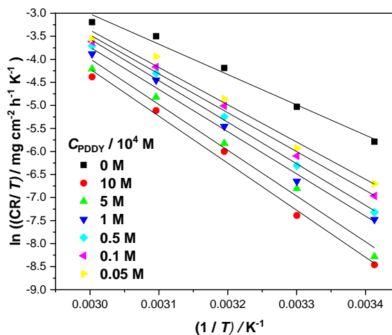
Figure 5. Transition state plots for mild steel corrosion rates in 1 M HCl in absence and presence of different concentrations of PDDY
