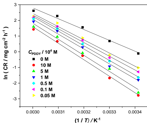
Figure 4. Plots for mild steel corrosion rates in 1 M HCl in absence and presence of different concentrations of PDDY
