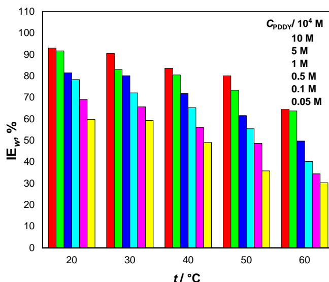
Figure 2. Variation of inhibition efficiency with temperature after 3 hours of mild steel exposure in 1M HCl and various concentrations of PDDY
