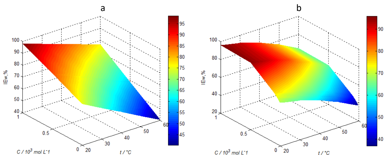
Figure 9. Surface plot for inhibition efficiency, temperature and inhibitor concentration based on: a) linear regression model; b) quadratic regression model
