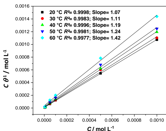
Figure 3. Langmuir adsorption plots for mild steel in 1 M HCl containing different concentrations of PDDY at various temperatures
