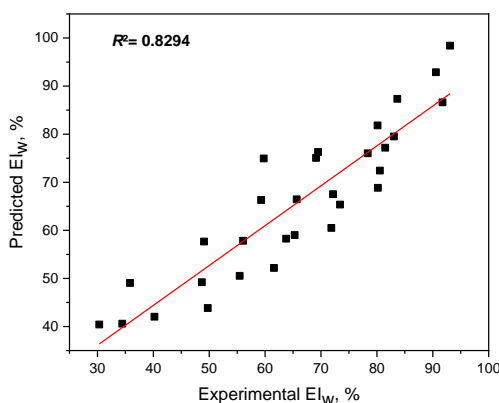
Figure 7. Fitting curves of predicted against experimental inhibition efficiency obtained by the linear regression model
