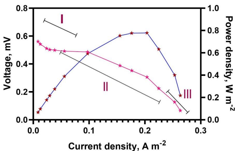
Figure 12. Polarization and power density graphs
