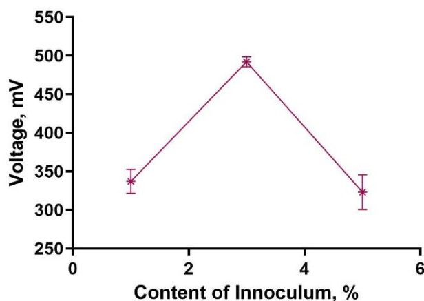
Figure 7. Effect of inoculum content on voltage generation.
