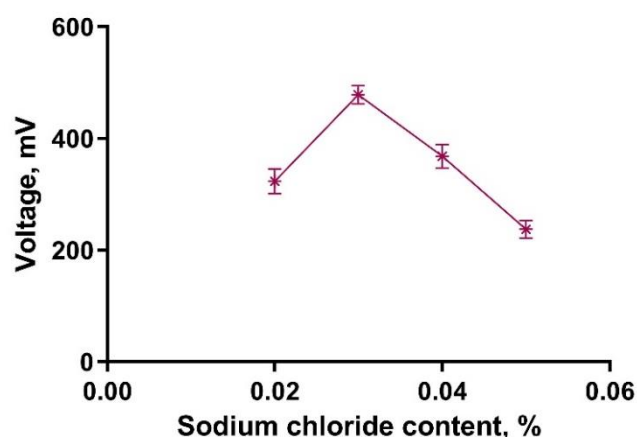
Figure 6. Effect of sodium chloride content on voltage generation
