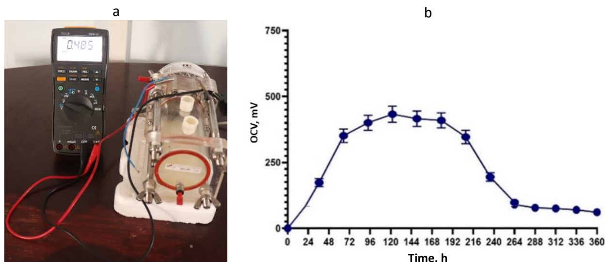
Figure 10. (a) Maximum voltage reached in batch operation of MFC with synthetic wastewater; (b) voltage vs. time in batch operation of MFC with synthetic wastewater
