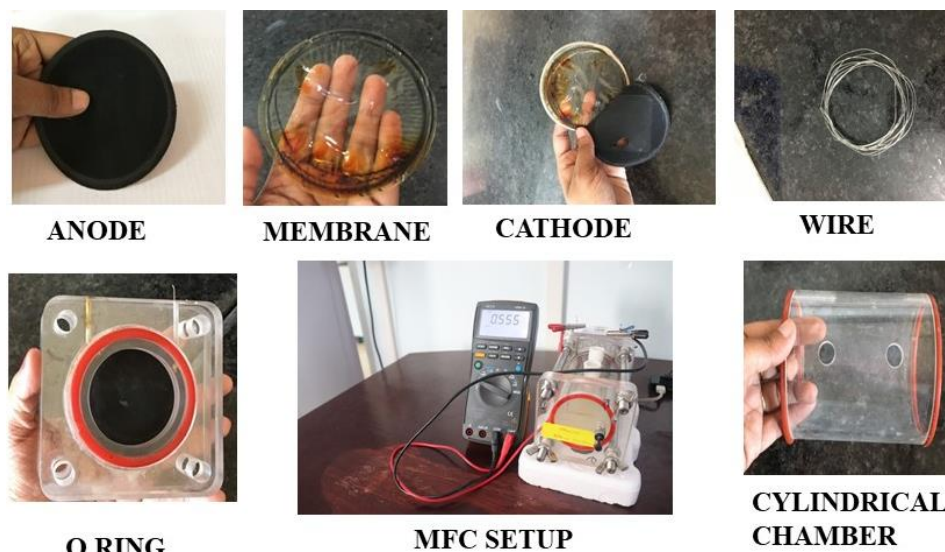
Figure 1. Single-chamber MFC components and setup
