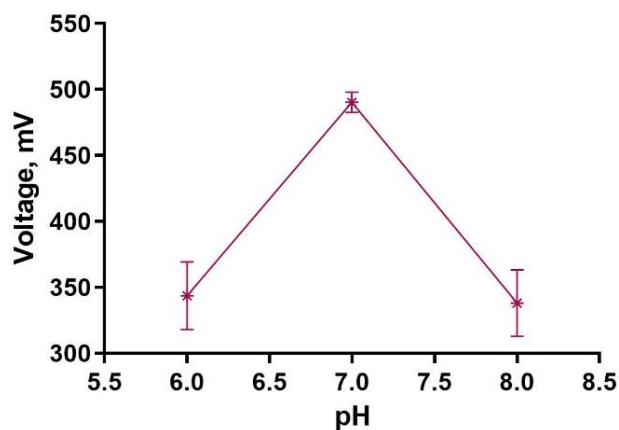
Figure 9. Effect of pH on voltage generation
