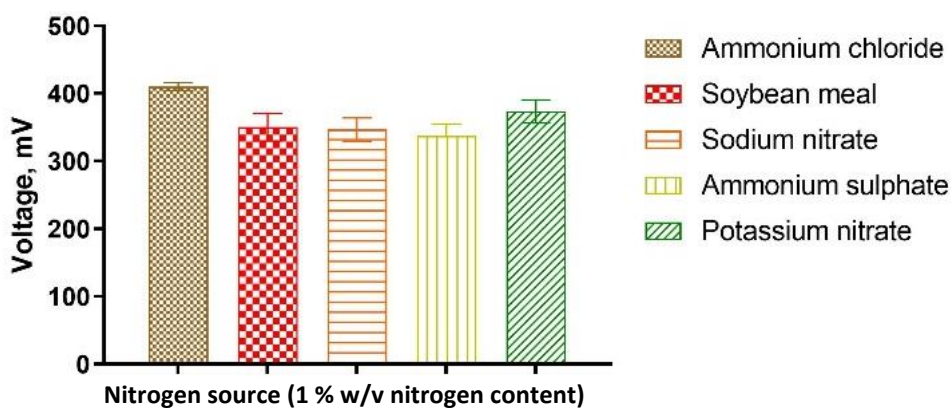
Figure 3. Effect of different nitrogen sources on voltage generation
