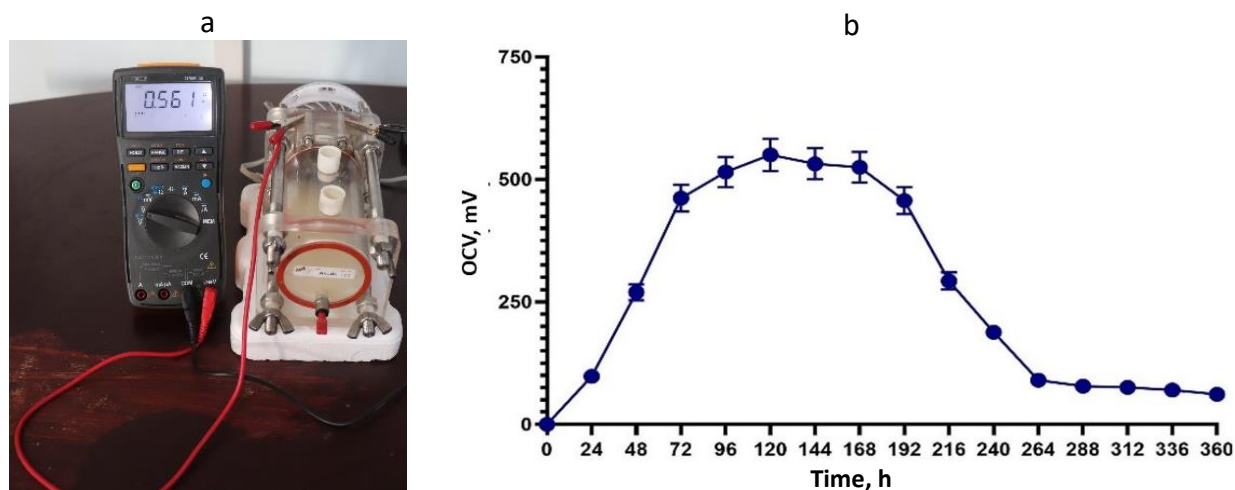
Figure 11. (a) Maximum voltage reached in batch operation of MFC with real dairy wastewater; (b) voltage vs. time in batch operation of MFC with real dairy wastewater
