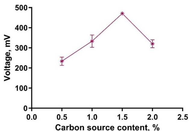
Figure 4. Effect of carbon content (lactose) on voltage generation
