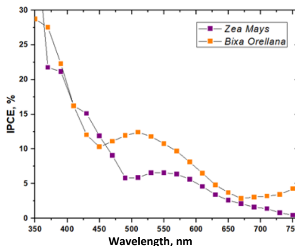
Figure 17. Incident-photon-to-current conversion efficiencies (IPCE) absorption spectra of DSSC utilizing dye extracted from purple corn and achote
